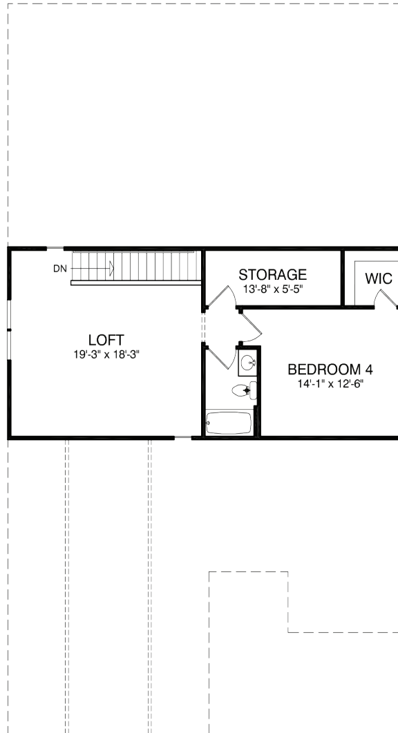
Optional Loft Floor Plan w/ Bedroom / Full Bath
