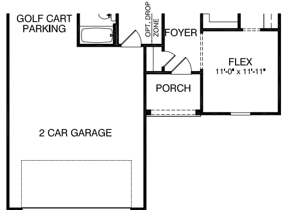
First Floor Plan w/ Opt. 4'-0" Garage Extension
