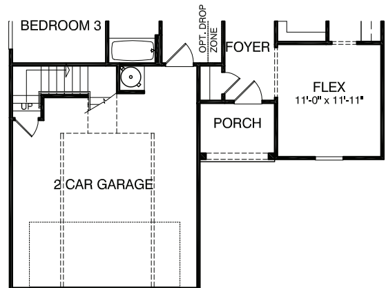
First Floor Plan w/ Opt. Bedroom 3 & Opt. Garage Attic Storage & 4'-0" Garage Extension
