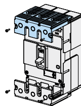
Assembly Diagram
