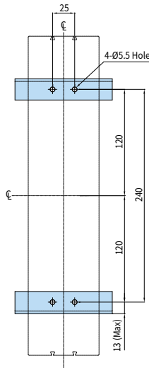
Mounting Drawing
