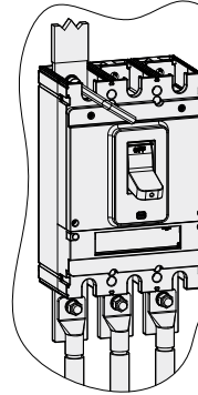
Terminal Connection
