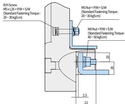
Detailed Drawing of Connection
