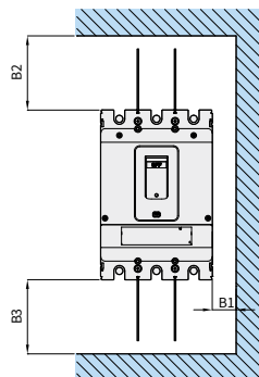
Up/down/left/right distance in case of metallic panel
