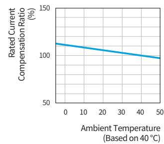
Ambient Temperature Derating Curve
