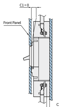
Front/back distance in case of metallic panel
