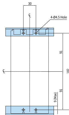
Mounting Drawing
