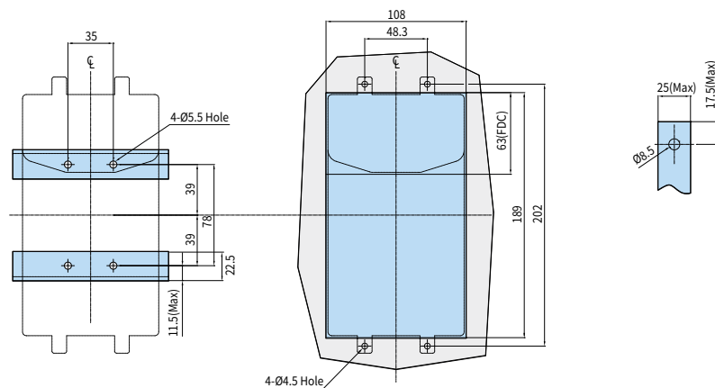
Process Criterion of Connecting Conductor
