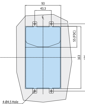
Dimension of Front Cover Cutting
