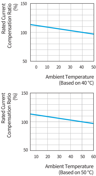
Ambient Temperature Derating Curve
