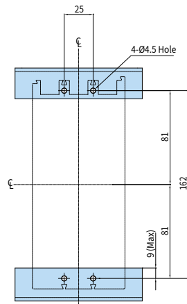
Mounting Drawing
