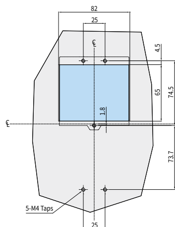
Mounting Drawing
