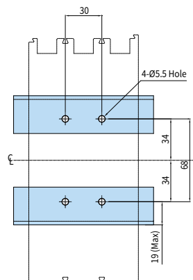
Mounting Drawing
