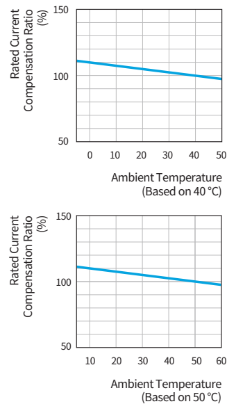
Ambient Temperature Derating Curve
