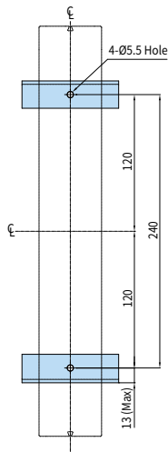
Mounting Drawing
