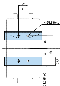
Mounting Drawing
