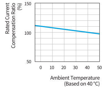
Ambient Temperature Derating Curve
