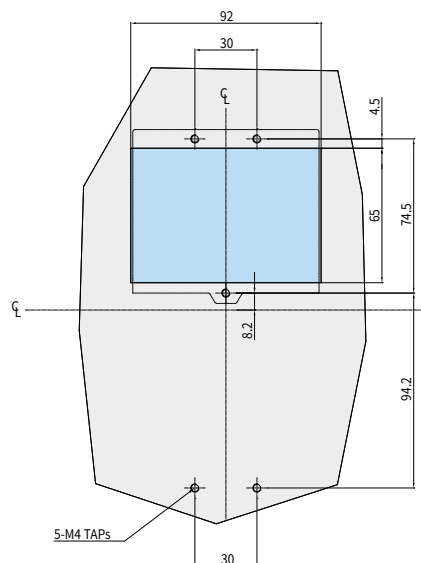
Mounting Drawing
