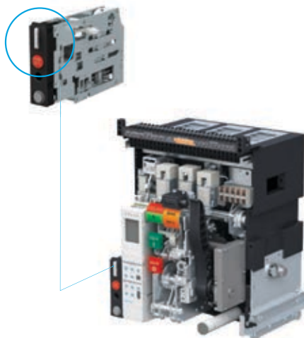
DR Device Unit & Position Pad Lock
