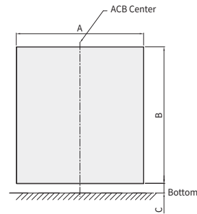
Rear Panel Cutting Size (For IP30)
