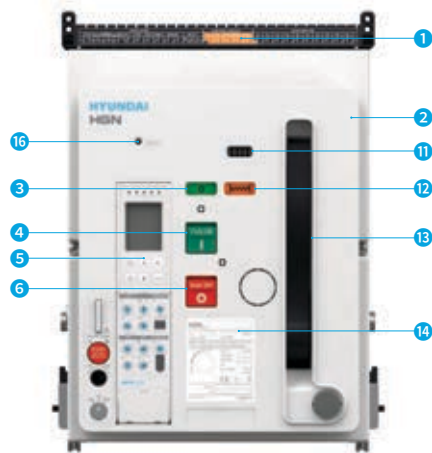
Draw-In/Out Type (ACB Body)
