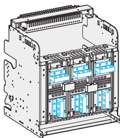
(Upper) Front Type + (Lower) Vertical Type
