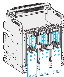
(Upper) Front Type + (Lower) Horizontal Type
