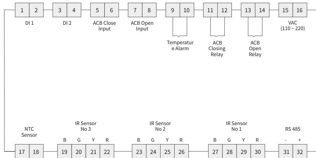
Block Diagram
