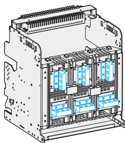
(Upper) Horizontal Type + (Lower) Front Type
