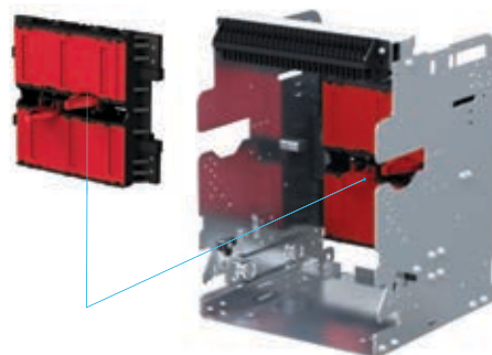
Safety Shutter & Shutter Lock
