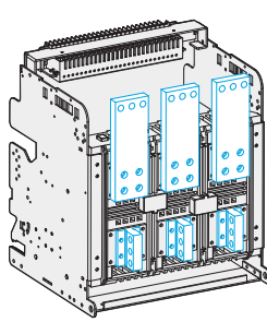
(Upper) Front Type + (Lower) Vertical Type
