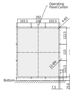
Panel Door Cut-Out (For Door Flange)
