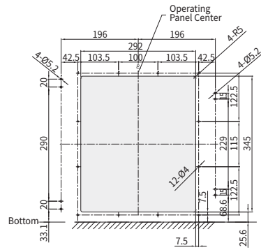
Panel Door Cut-Out (For Dust Cover)
