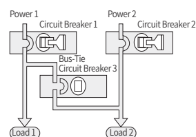
Circuit Breaker 3 cannot be closed
