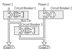
Circuit Breaker 2 cannot be closed
