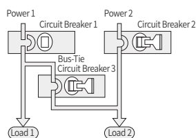
Circuit Breaker 1 cannot be closed
