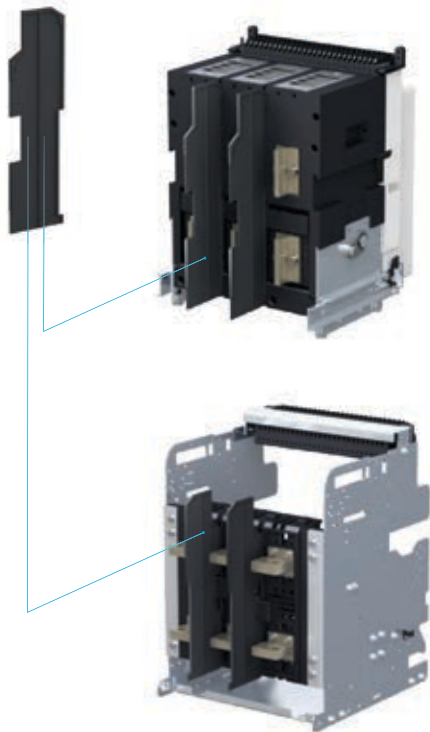
Phase Insulation Barrier
