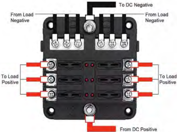
BLADE FUSE BLOCK WIRING DIAGRAM 6 Circuits with Negative Bus
