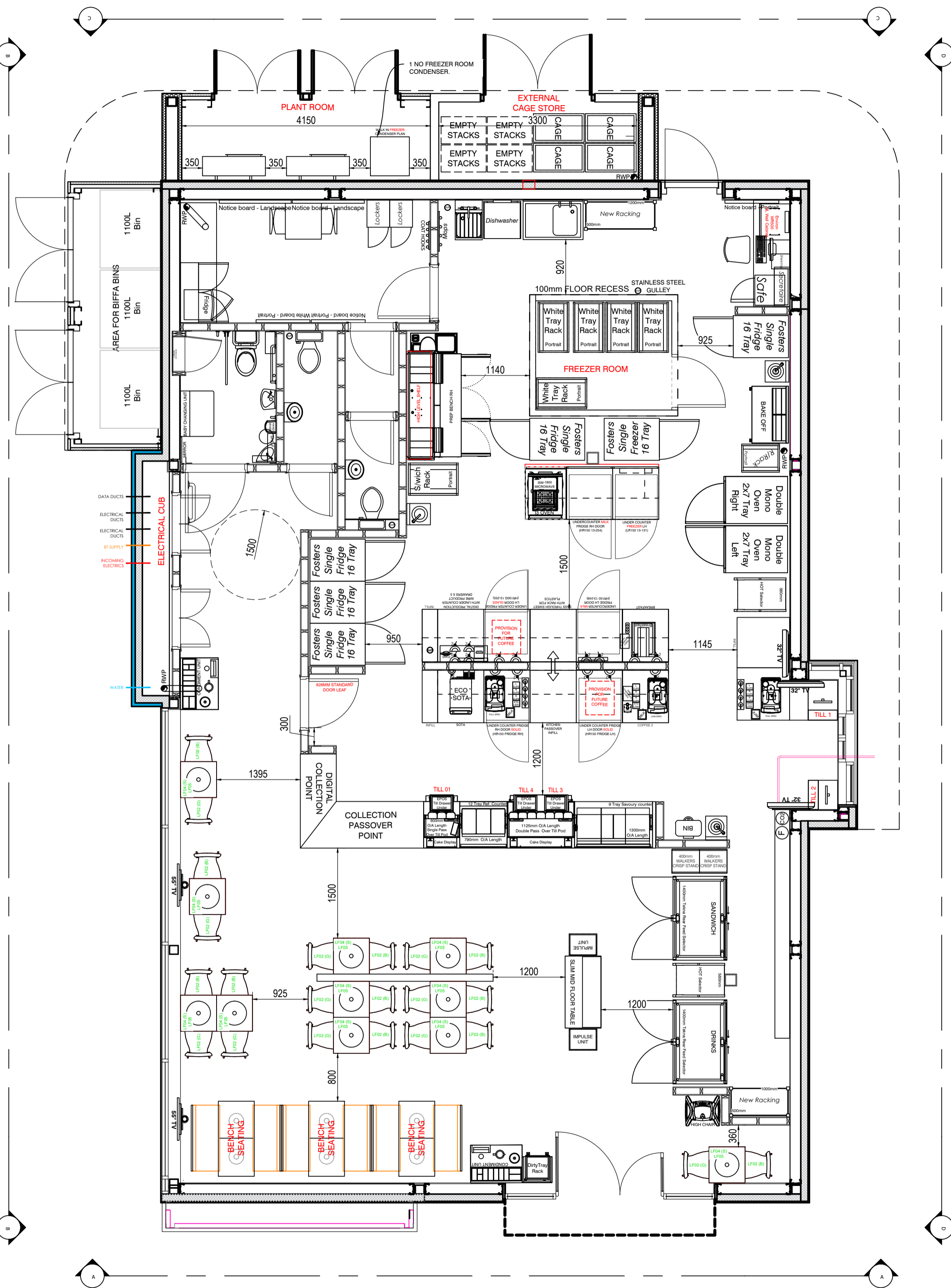
PROPOSED BLOCK PLAN GA (1:50)
