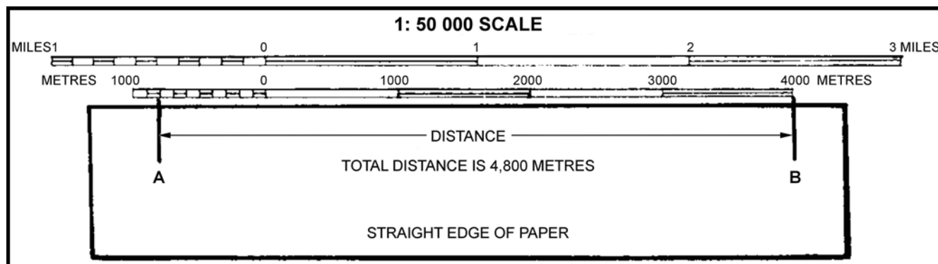
Figure 16-6-2 Calculating Distance
