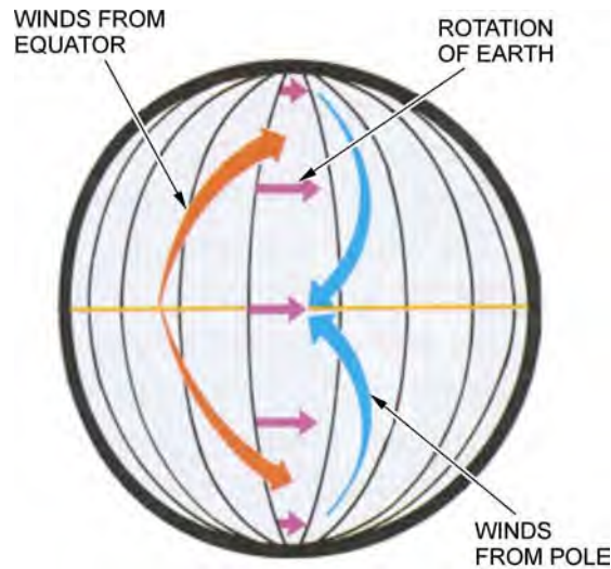
Figure 14-4-7 Coriolis Effect
