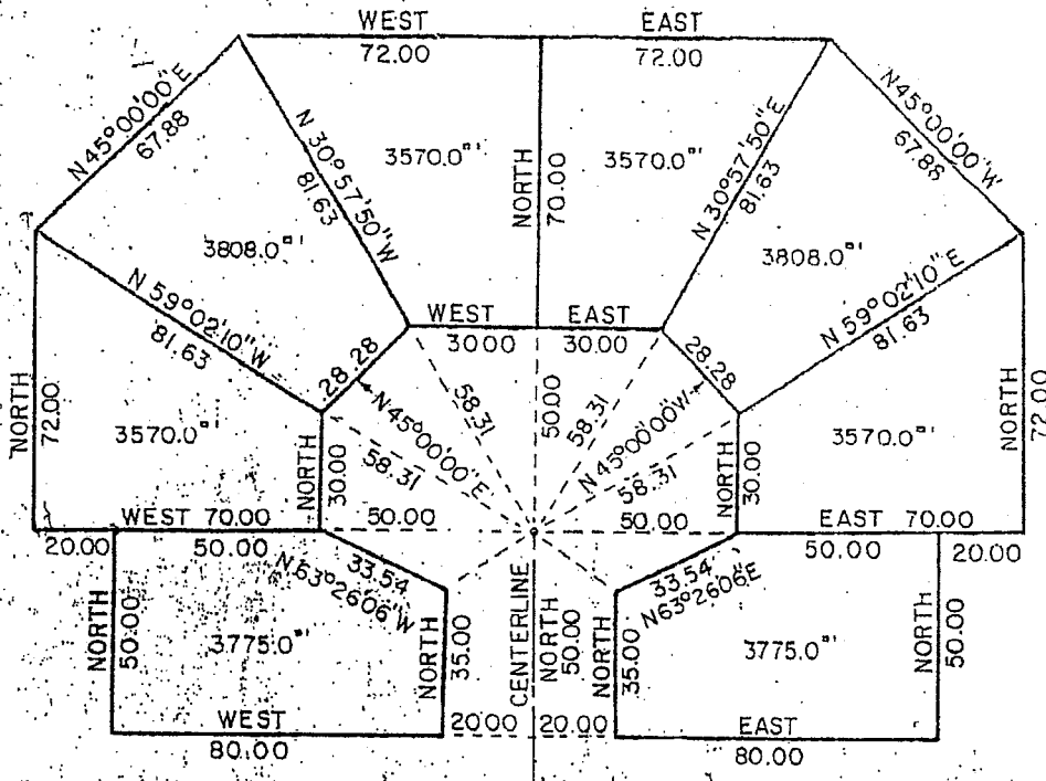
TYPICAL LOT CLUSTER
