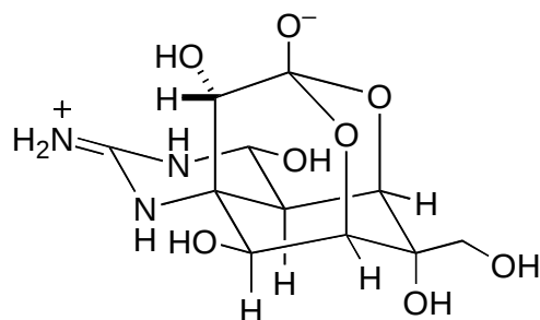
tetrodotoxin ( 1 )
