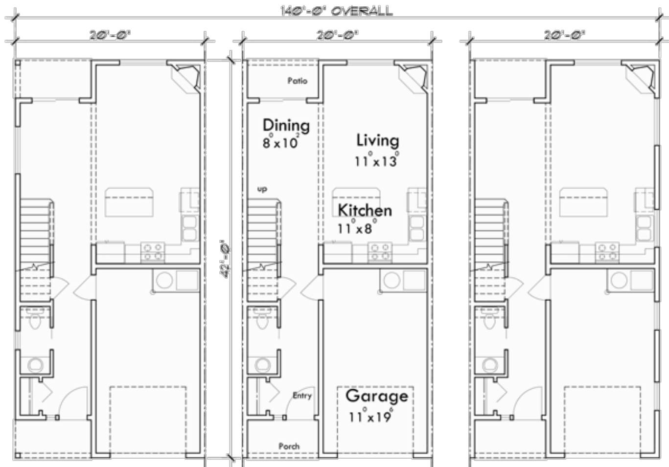
Main Floor Plan "Unit D"
