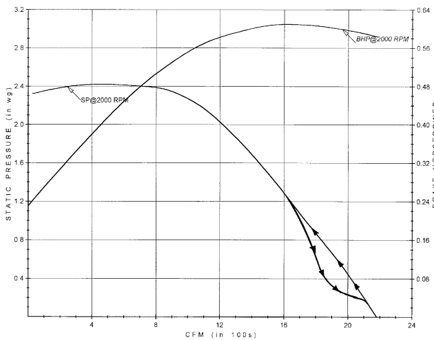
Figure 7. Bi-Stable Flow
