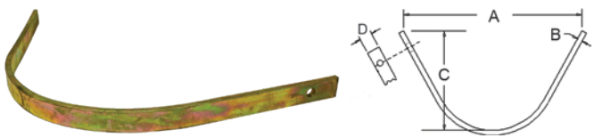
A-RRT1 Rock Rake Tooth .375" mounting hole A - 17" B - .315" C - 9 5/8" D - 1"
