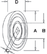
A-VLH6706 Washer, Large For 1" Axles, Cast Iron, Painted Black A: 6.437" B: 1.750" C: 1.062" D: 1.125"
