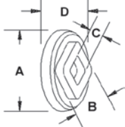
A-VLH6705 Washer, Small For 1" Axles, Cast Iron, Painted Black A: 3.562" B: 1.875" C: 1.062" D: 1.312"
