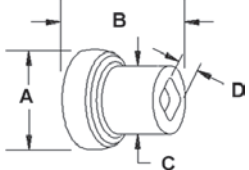
A-VLH6709 Spool Spacer 3-5/8" For 1" Axle, Cast Iron, Painted Black A: 3" B: 3.312" C: 2.250" D: 1.000"
