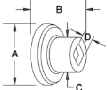
A-VLH6708 Spool Spacer 2-3/8" For 1" Axle, Cast Iron, Painted Black A: 4" B: 2.375" C: 2.250" D: 1.125"
