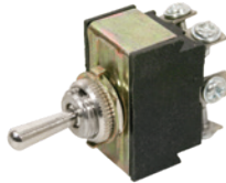
A-L5592 Switch, Universal, Toggle Position: 3 Terminal: 6 Thread: 7/16" Mounting Stem Type: Toggle
