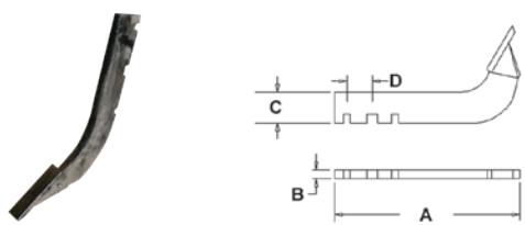
A-BSS2534BN Box Scraper Shank w/ Point .562" notches in shanks back A: 15.250" B: .750" C: 2.5" D: 3.625"
