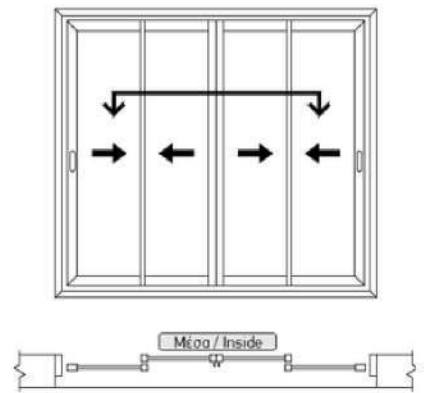
Cross Section 4 Pane
