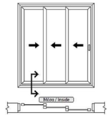
Cross Section Triple Track
