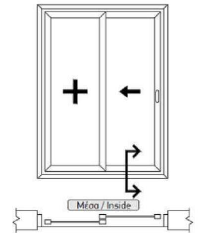
Cross Section Double Track
