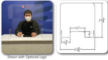
Sneeze Guard-A-24x24: (Part#: CI-SG-A-2x2)
