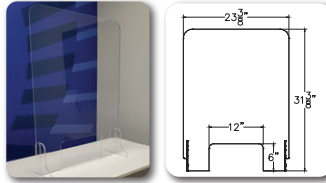
Sneeze Guard-A-24x32: (Part#: CI-SG-A-2x2.5)
