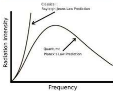
Blackbody Radiation vs Frequency
