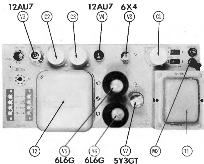
POWER AMP CHASSIS TOP VIEW
