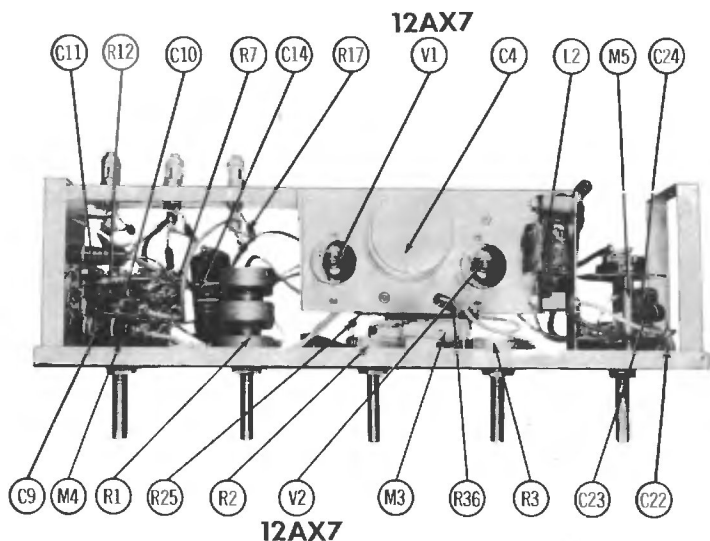
PRE-AMP CHASSIS TOP VIEW
