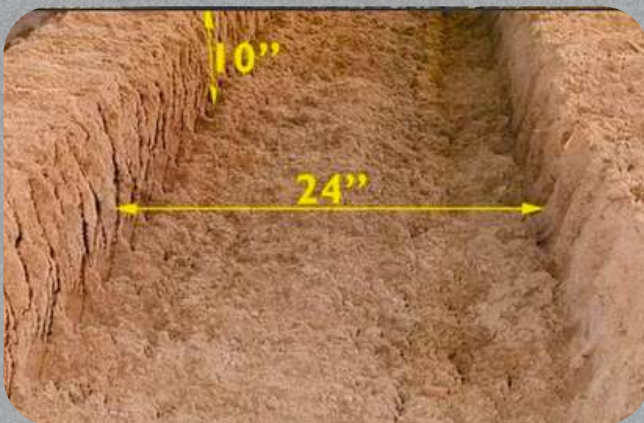
FINISHED TRENCH
