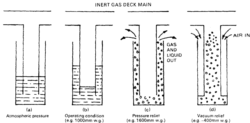
Figure 16 Principles of liquid-filled pressure/vacuum breakers.
