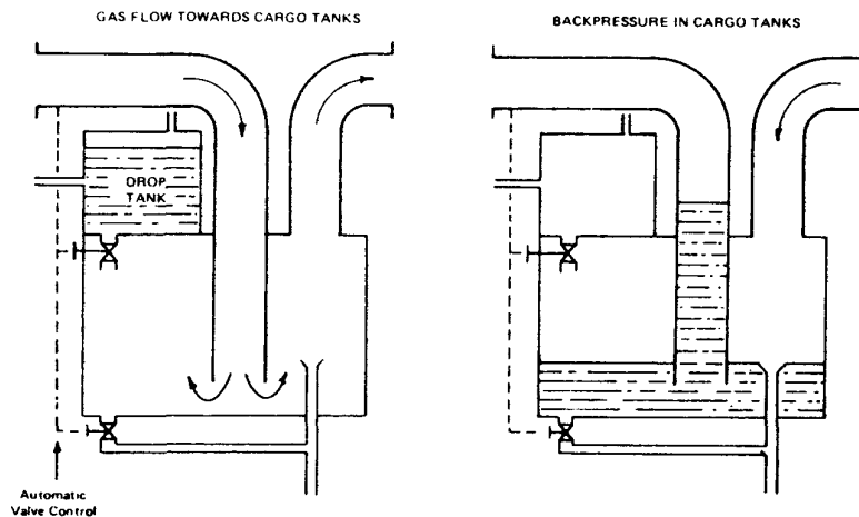
Figure 9 Deck water seal – dry type.
