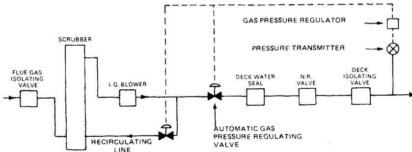
Figure 10 Typical automatic pressure control system.
