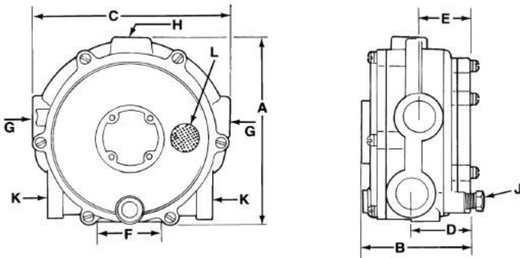
C-COBRA REGULATOR DIMENSIONS
