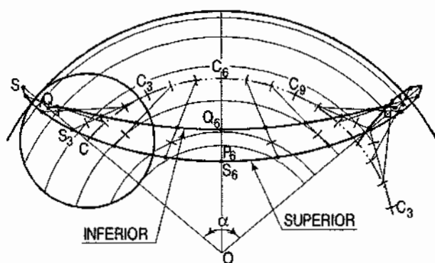
Hypotrochoids
