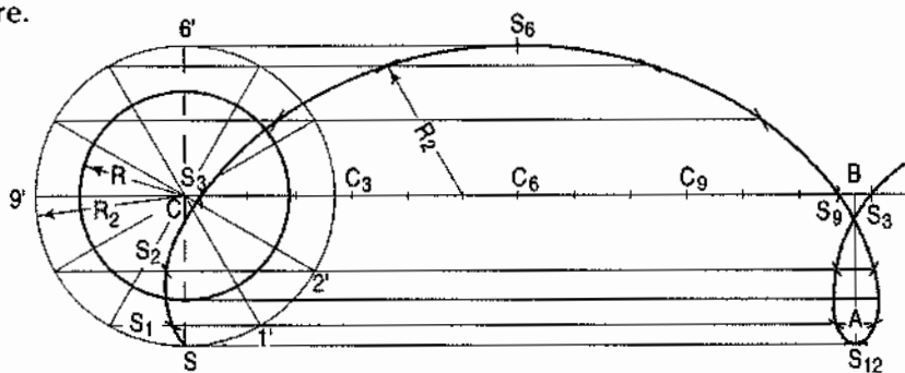
Superior trochoid
