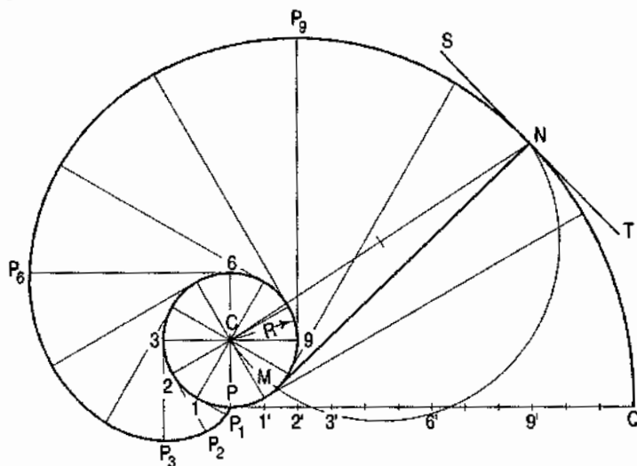
Involute
