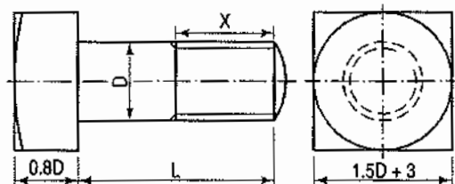
Square-headed bolt
