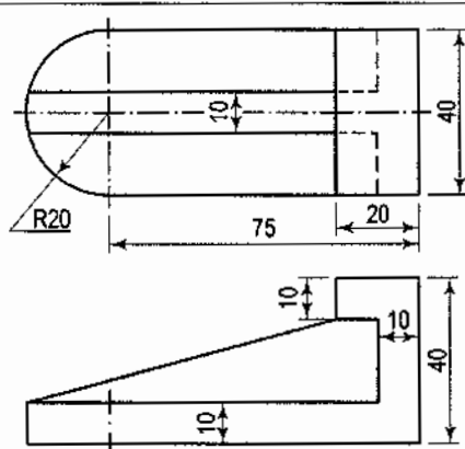
(Third-angle projection)
