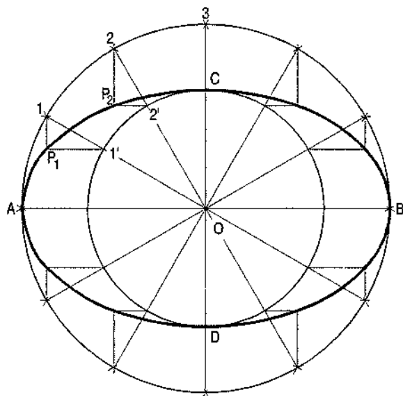
Concentric circle method
