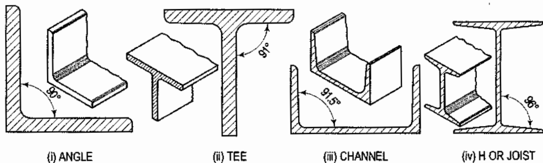
Rolled-steel sections
