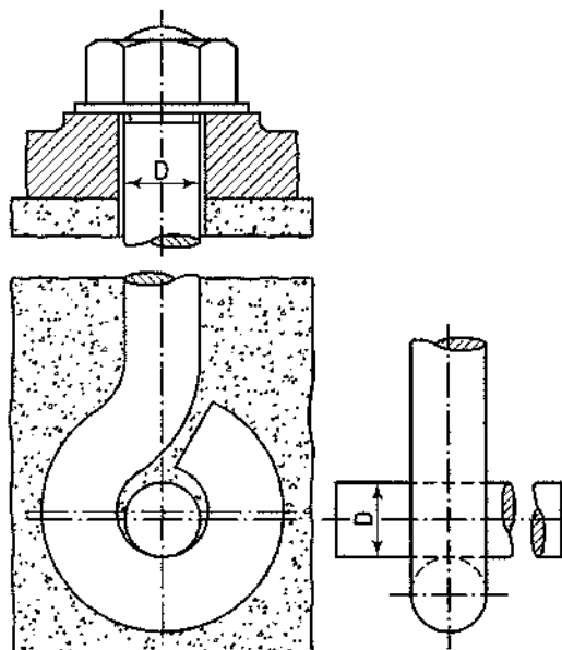
Eye bolt FIG. 24-66
