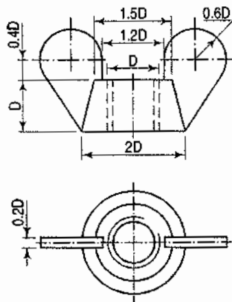
Wing nut
