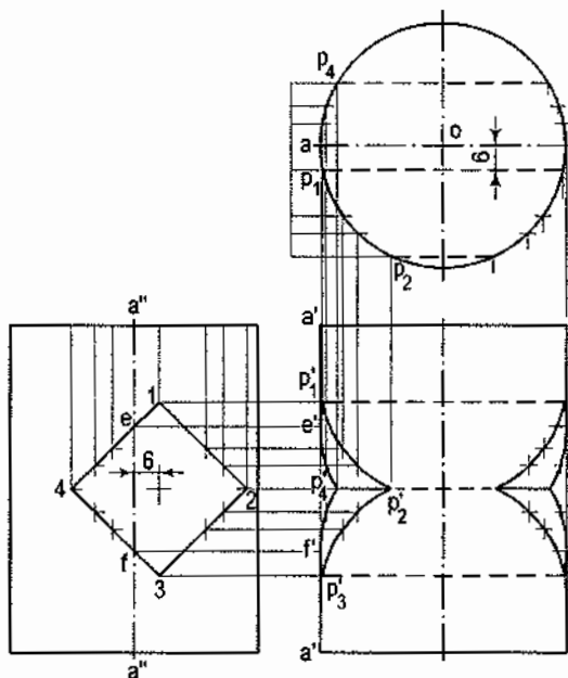
(Third-angle projection)
