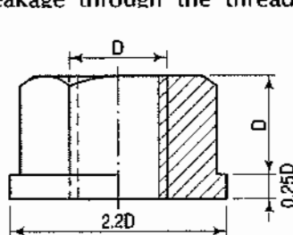
Flanged nut FIG. 24-7
