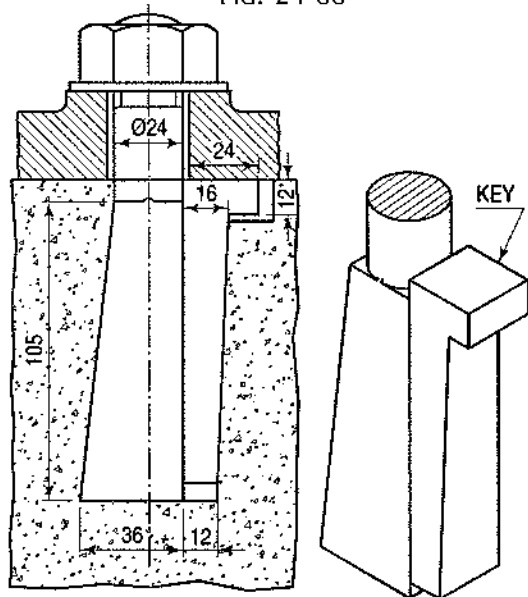
Lewis bolt FIG. 24-68
