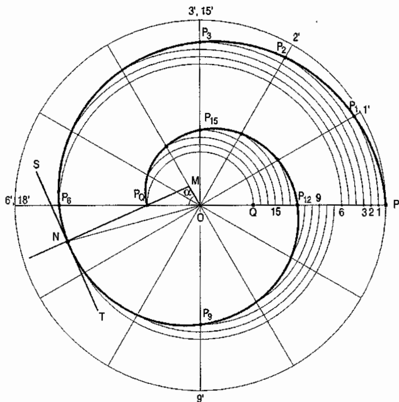
Archimedean spiral
