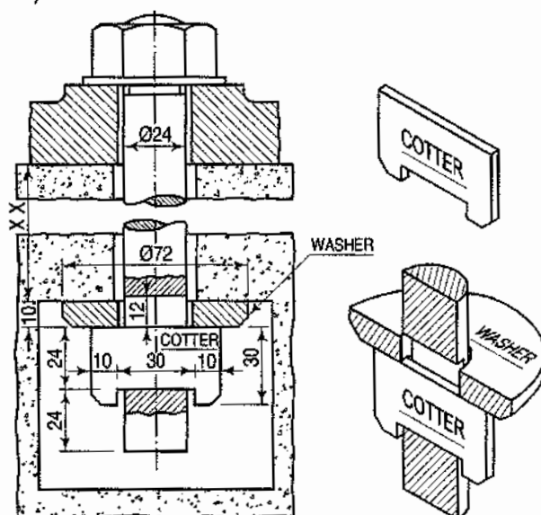
Cotter bolt
