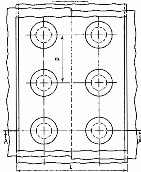
Single-riveted (double straps) butt joint FIG. 25-10
