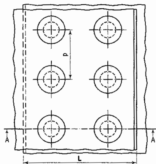
Double-riveted (chain) lap joint
