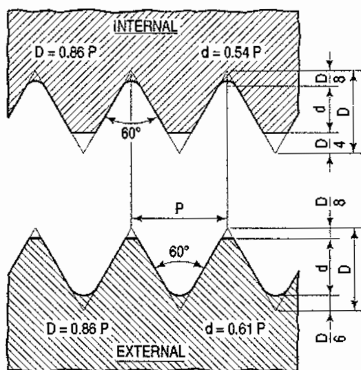
Unified thread
