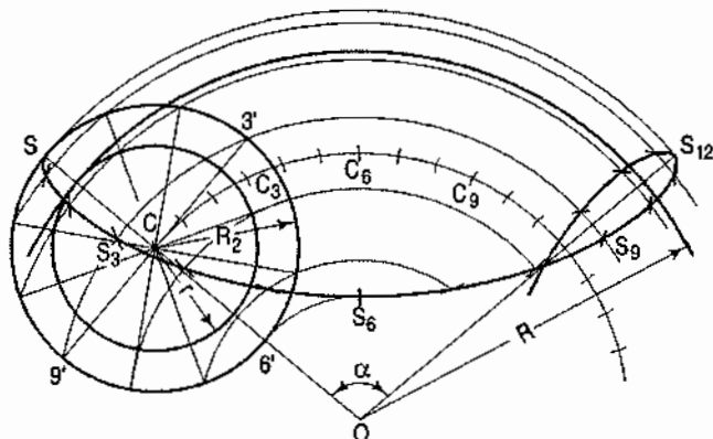
Superior hypotrochoids
