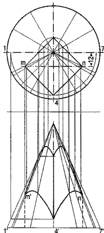
(Third-angle projection)
