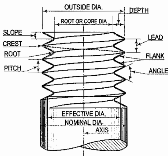
Screw thread FIG. 23-1
