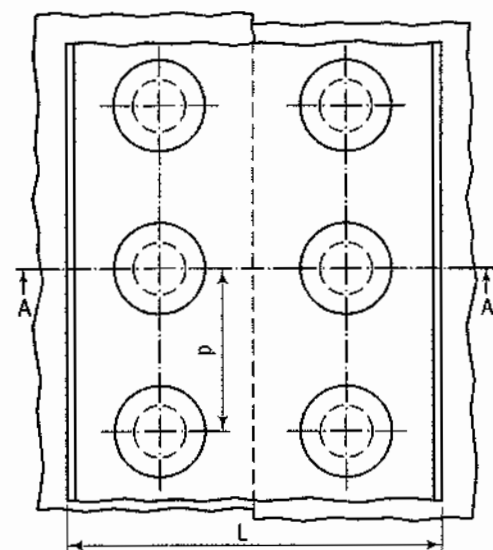
Single-riveted (single strap) butt joint FIG. 25-9
