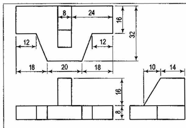
(Third-angle projection)
