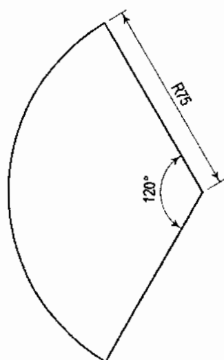
(i) DEVELOPEMENT OF CONE
