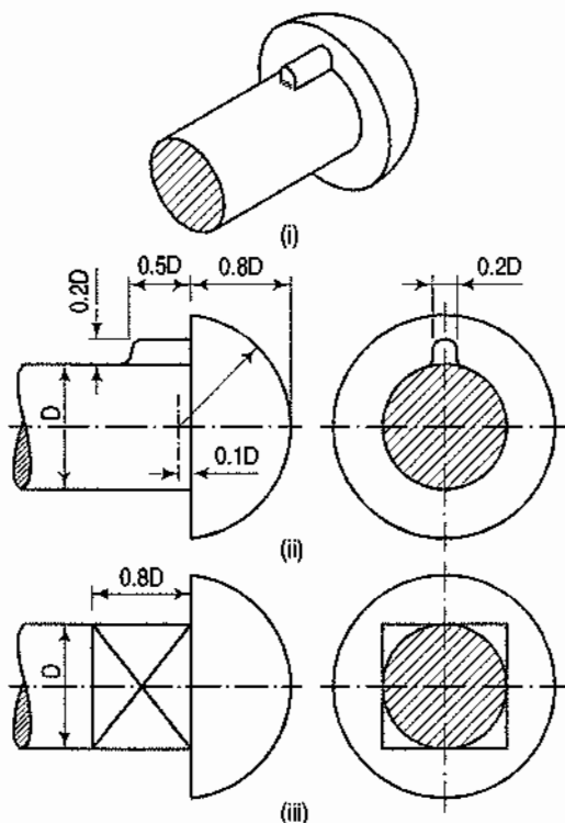
Cup-headed bolt
