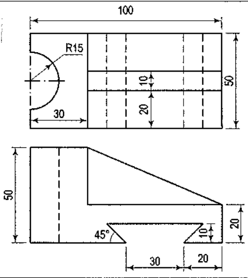
(Third-angle projection) FIG. 17-105
