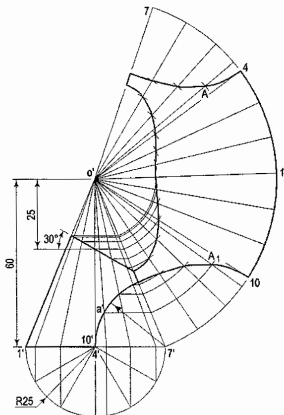
FRONT VIEW OF CONE
