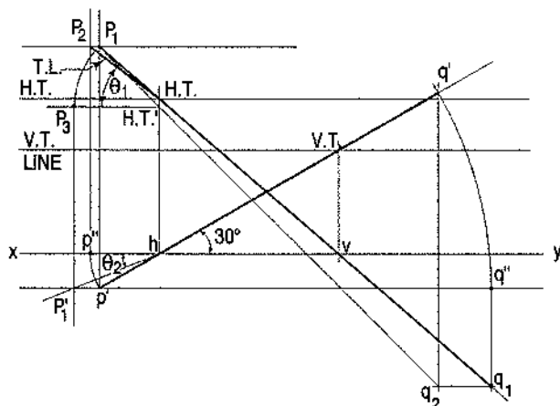
T.L. = 25 mm. \angle V.P., \theta_1 = 37^\circ \angle V.P., \theta_2 = 22^\circ FIG. 10-51
