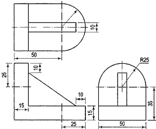
(Third-angle projection) FIG. 17-49
