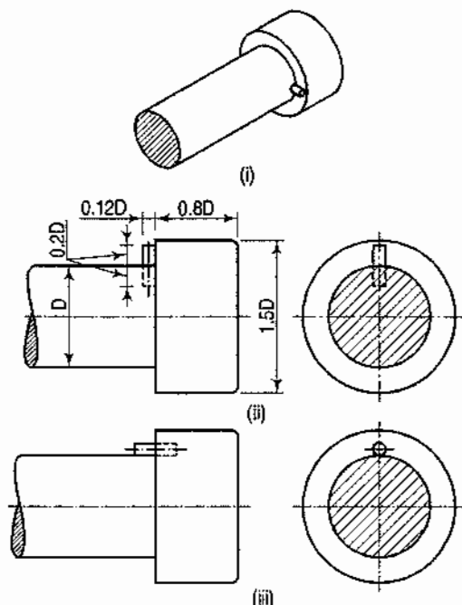
Cylindrical or cheese-headed bolt
