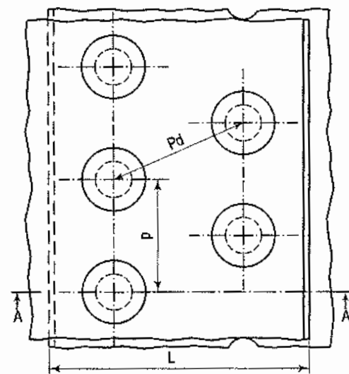
Double-riveted (zigzag) lap joint
