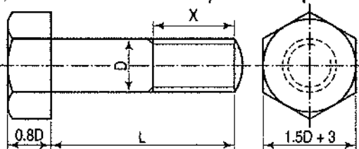
Hexagonal-headed bolt – approximately standard dimensions FIG. 24-15
