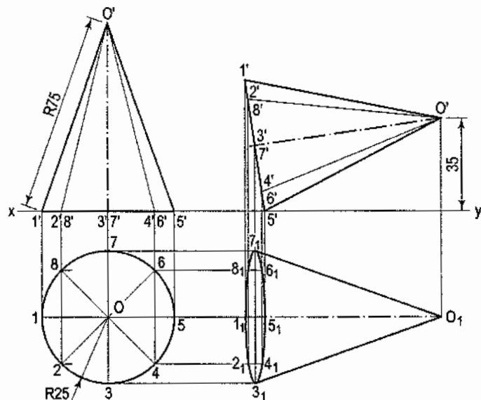
(ii) CONE AND PROJECTIONS GENERATED FROM DEVELOPEMENT OF CONE
