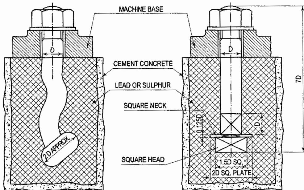
Curved or bent bolt
