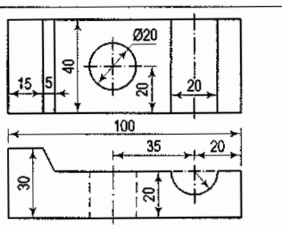
(Third-angle projection)
