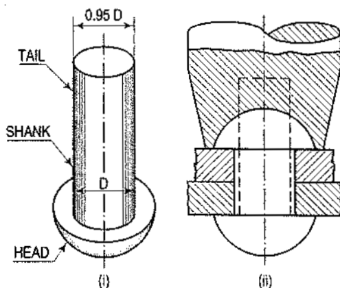
Rivet and riveting FIG. 25-1
