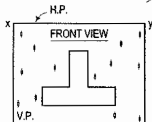
THIRD-ANGLE PROJECTION
