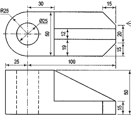
(Third-angle projection) FIG. 17-51
