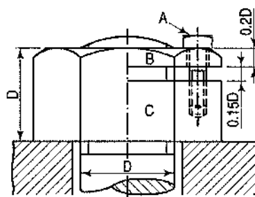
Sawn nut
