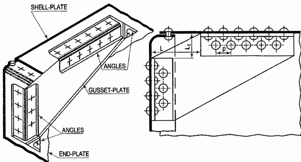
Gusset stay
