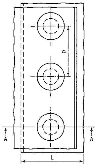
Single-riveted lap joint
