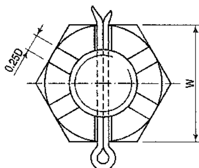
Castle nut
