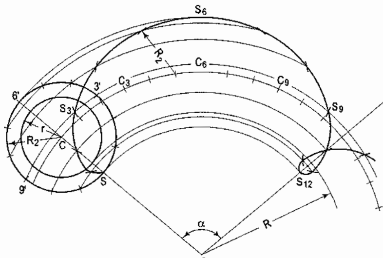
Superior epitrochoid
