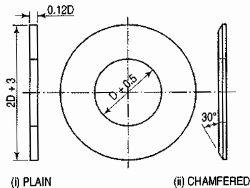
Washers
