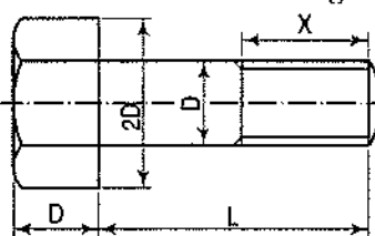
Hexagonal-headed bolt – rough-rule dimensions FIG. 24-14
