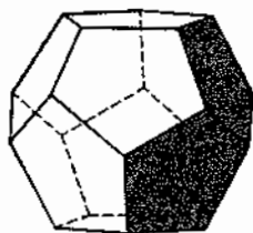
Dodecahedron FIG. 13-4
