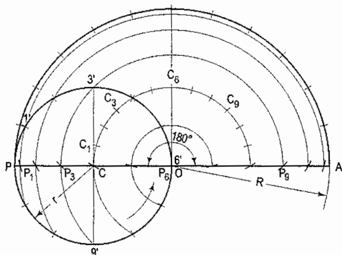
Hypocycloid
