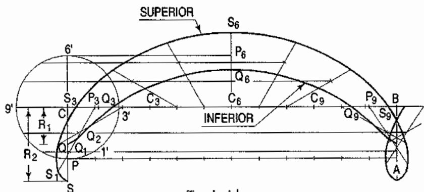
Trochoids
