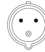
IEC 60309, 2P 3W, 6H IP44(SPLASHPROOF) 32A, 240V MAX RATED INPUT
