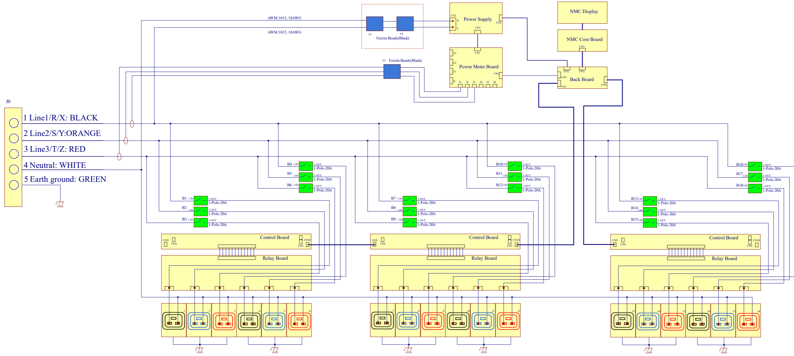
INTERNAL WIRING SCHEMATIC
