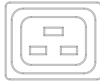
IEC 60320/C19 16A,250V MAX RATED OUTPUT
