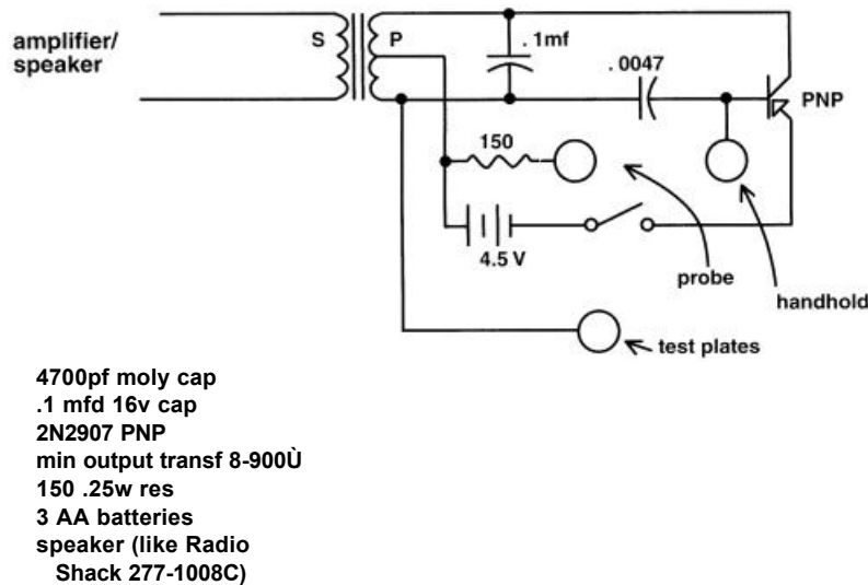
Fig. 79 Syncrometer schematic.
