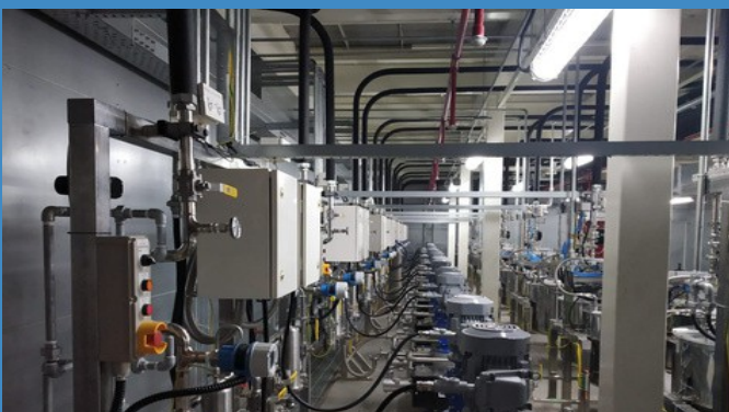
Paint Circulation System-Maruti Suzuki
