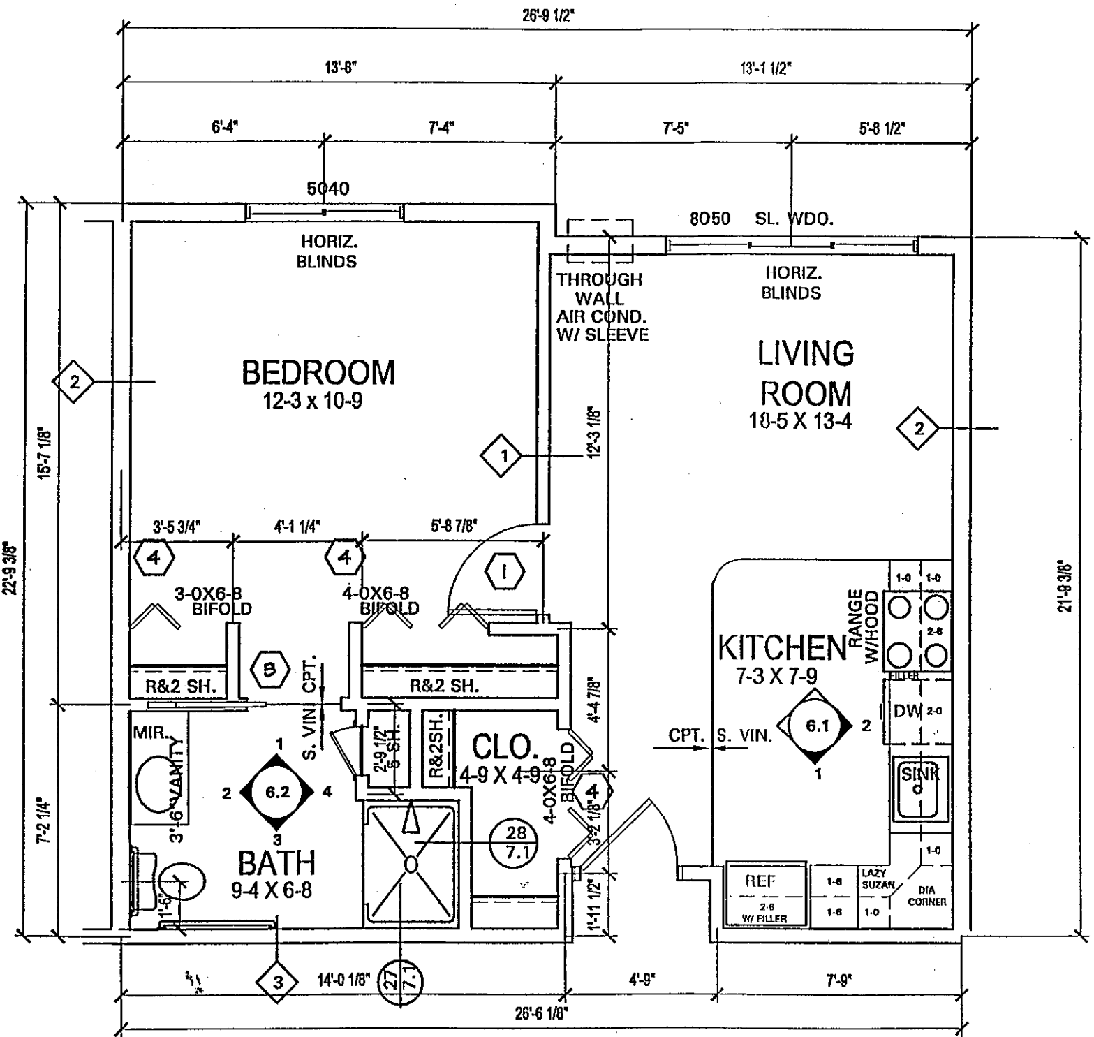
UNIT-C 1 BEDROOM SCALE 1/4" = 1'-0"
