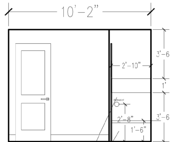
ELEVATION D
