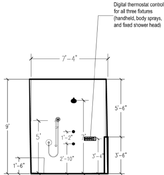
ELEVATION C
