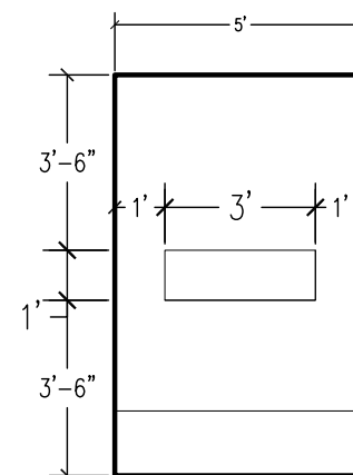
ELEVATION D
