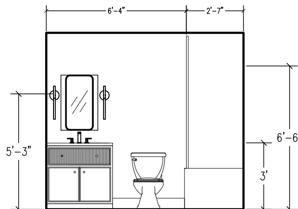
ELEVATION C
