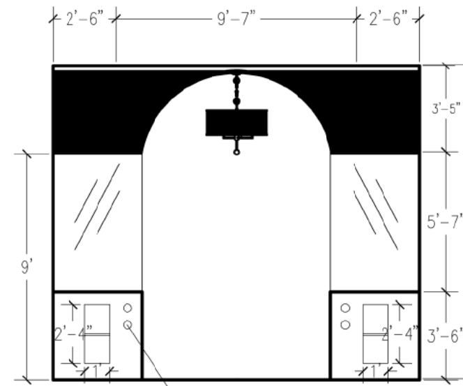
ELEVATION D
