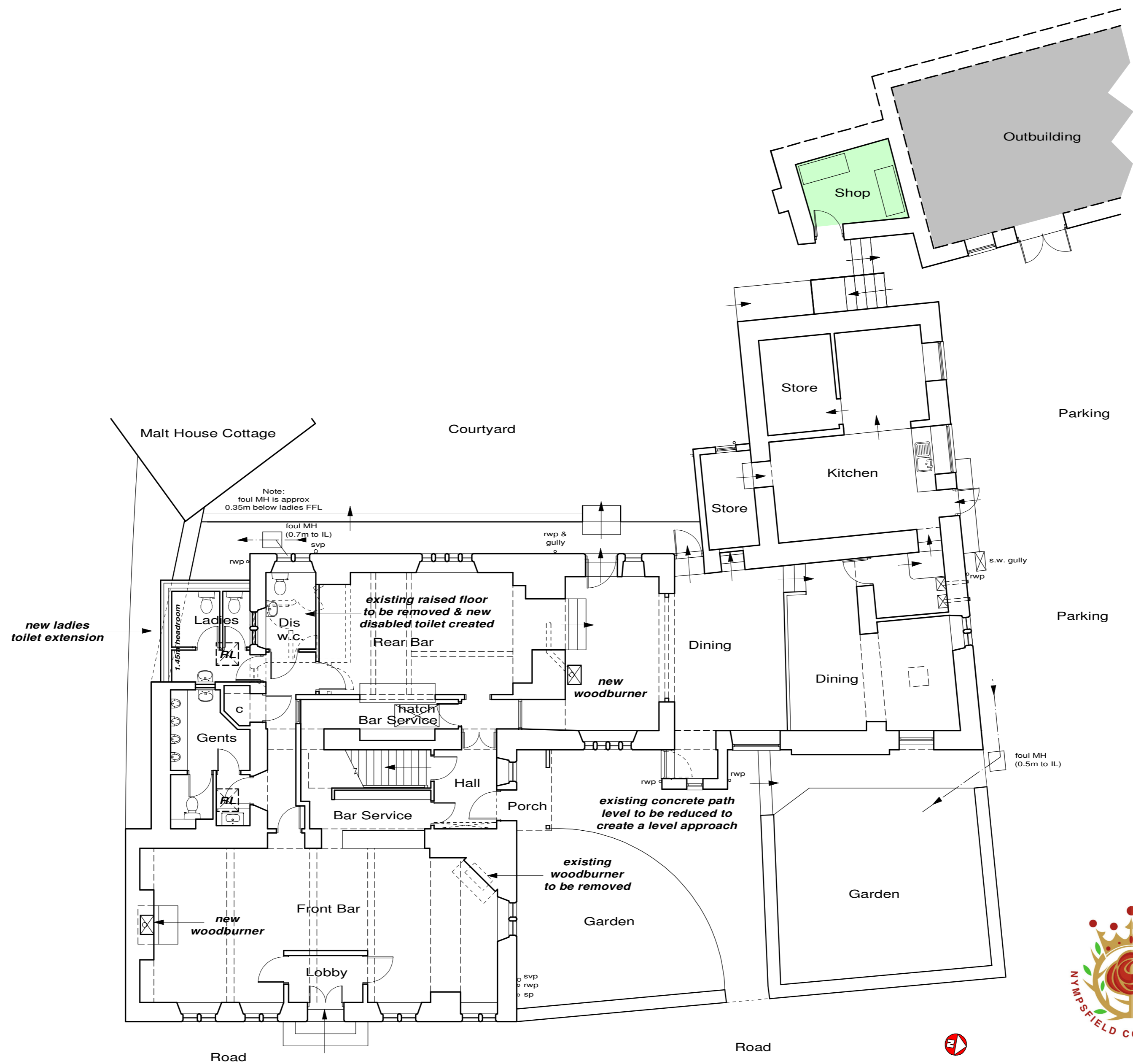
PROPOSED GROUND FLOOR PLAN/PART SITE PLAN 1:100
