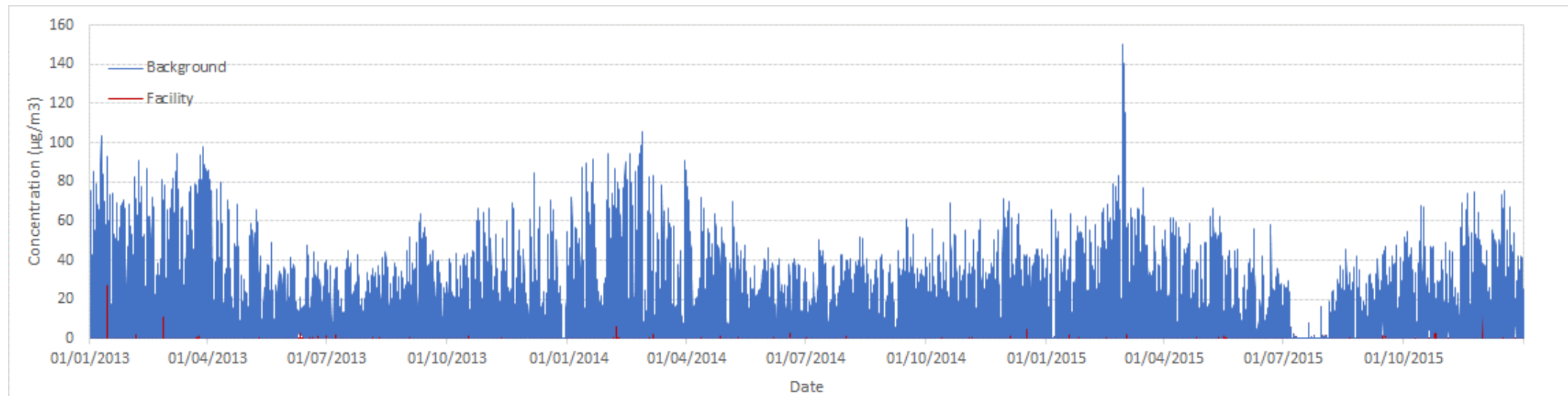
FIGURE 7.4 FROM THE AQTR: HOURLY TIME SERIES OF MODELLED NO 2 CONCENTRATIONS AT PLAZA 400, SHOWING BACKGROUND AND FACILITY CONTRIBUTION
