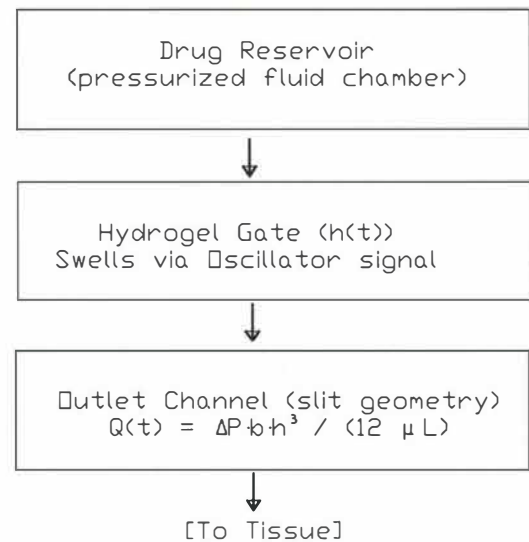
Fig. 4 - Device Schematic (Self-Tuning Capsule)
