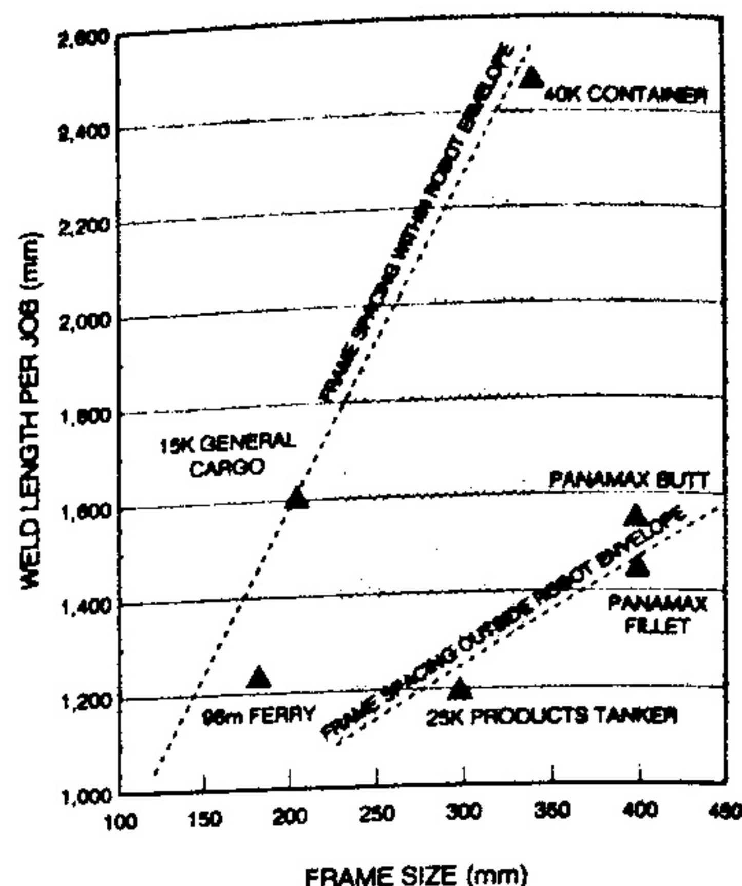
Fig. 2 Effect of ship size on weld length per job
