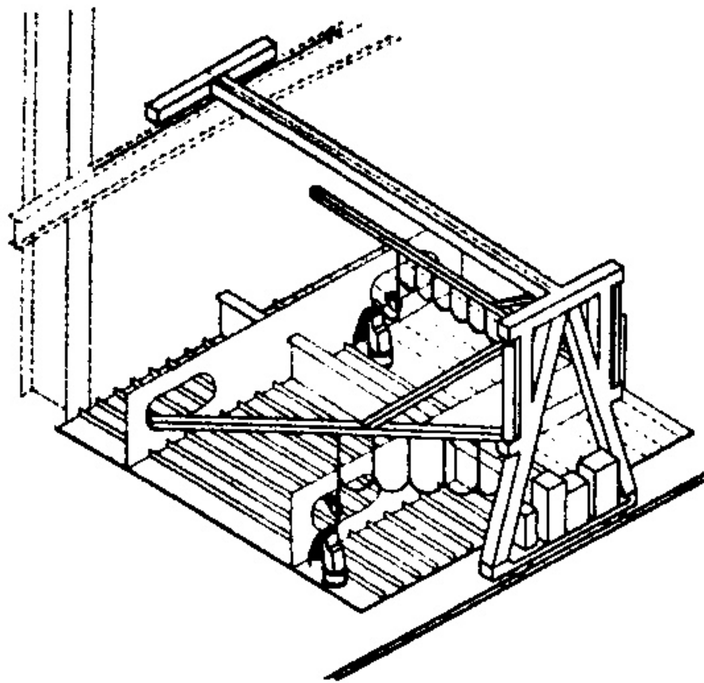
Fig. 8 Robot handling aid for vertical access
