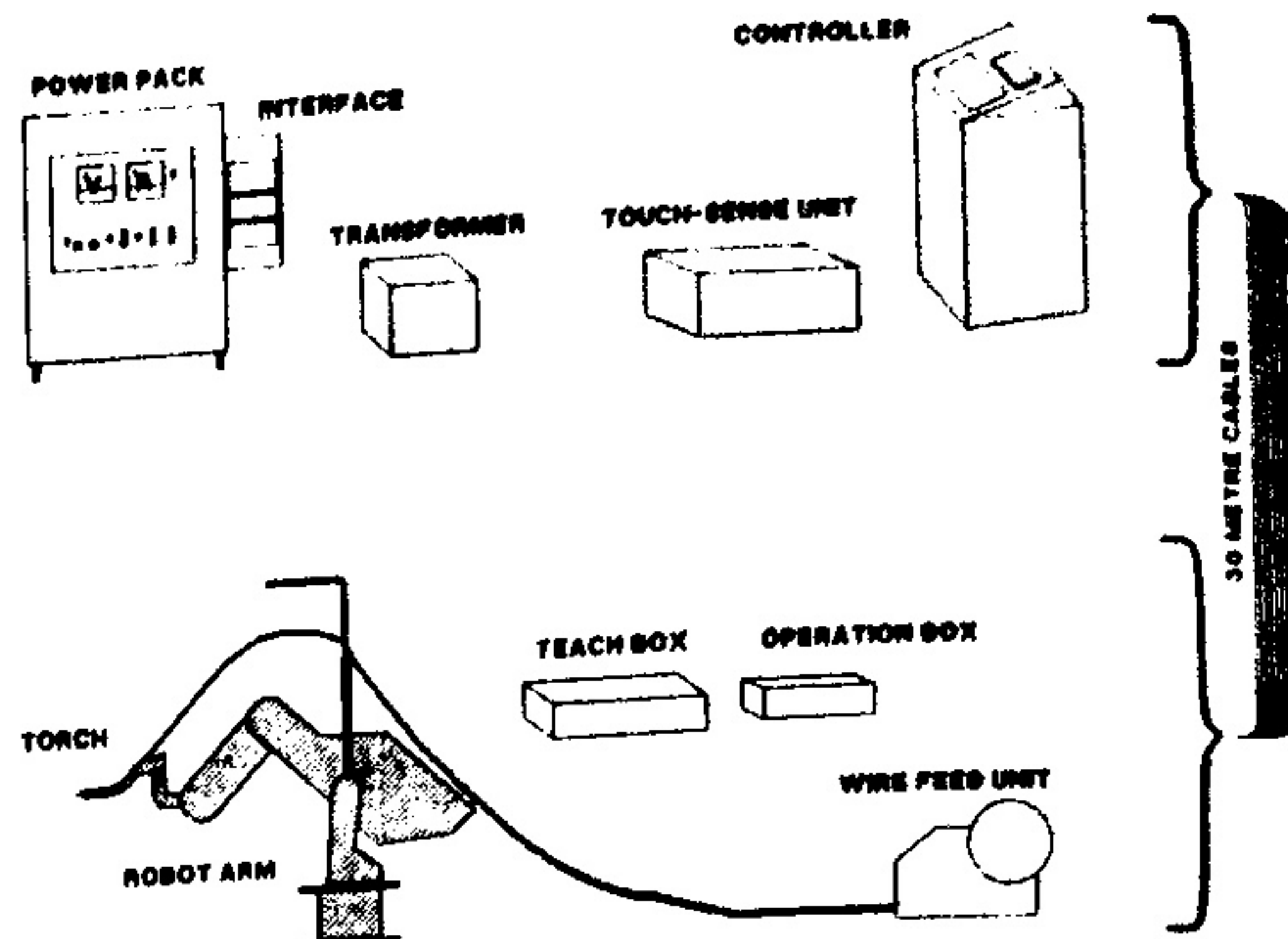
Fig. 7 Hitachi M5030Z system components
