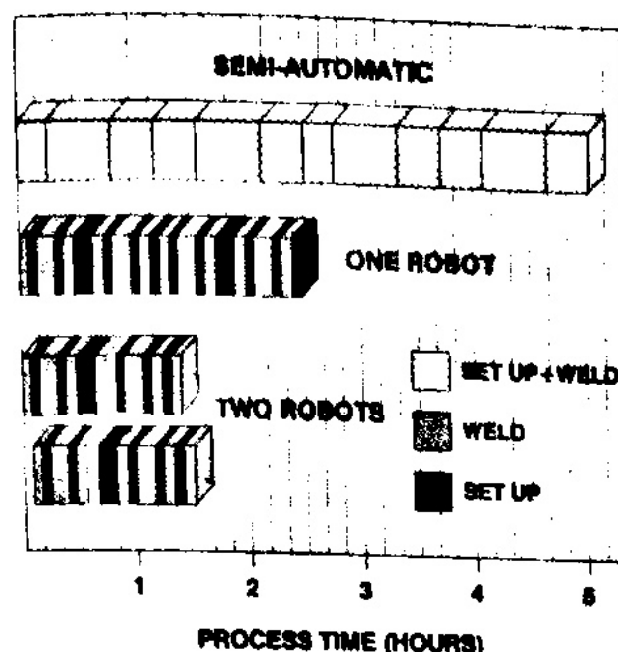
Fig. 3 Comparison of process times for one watertight bulkhead
