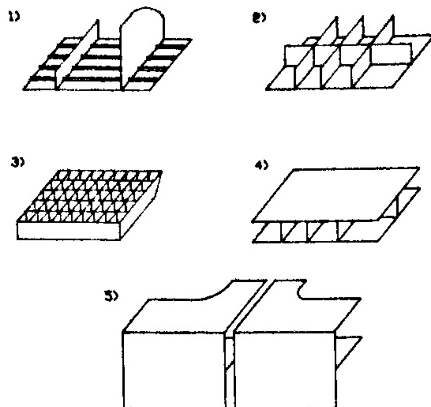
Fig. 6 Initial assembly types for robotic welding
