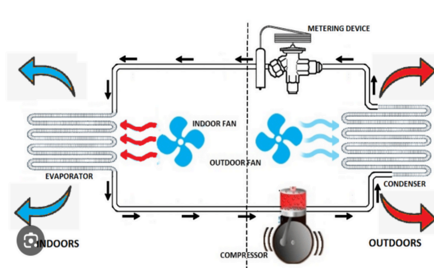
Basic Refrigeration System
