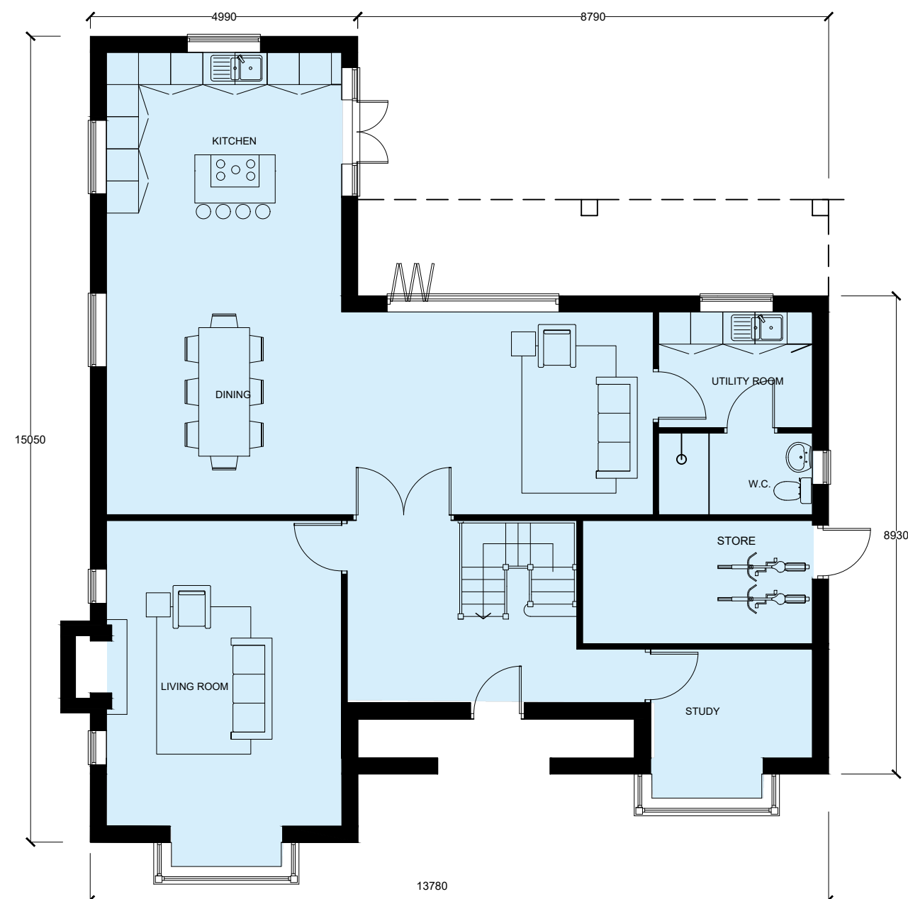
GROUND FLOOR PLAN TYPE 4: 341 m2
