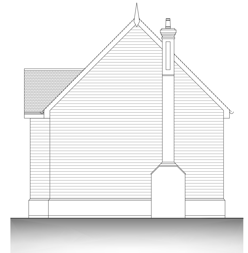
SIDE ELEVATION
