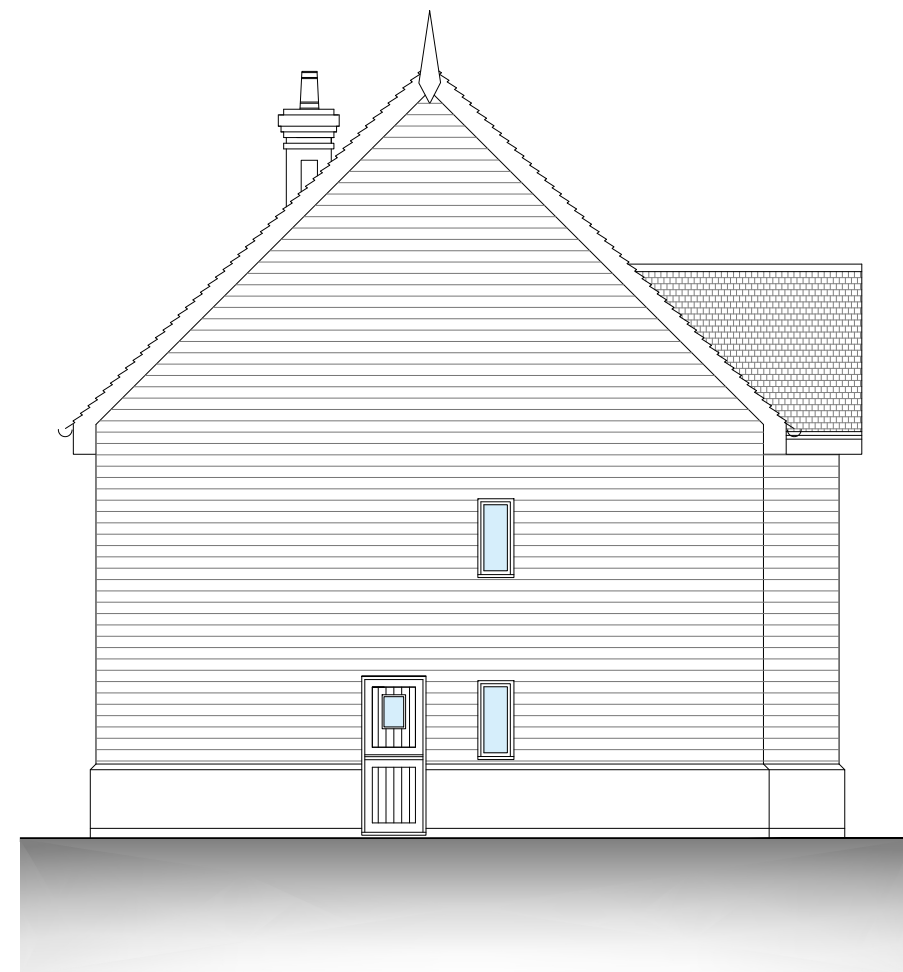
SIDE ELEVATION
