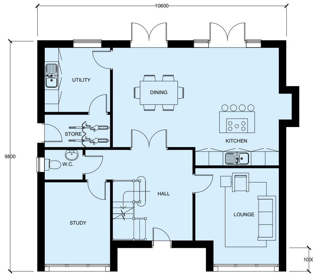
GROUND FLOOR PLAN TYPE 8: 266 m2
