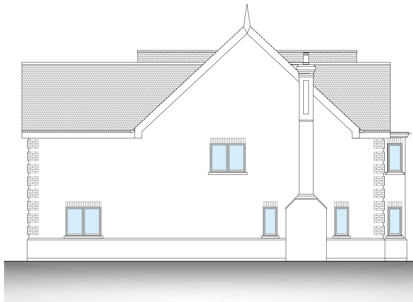
SIDE ELEVATION
