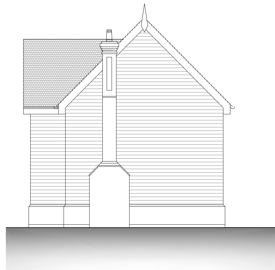
SIDE ELEVATION
