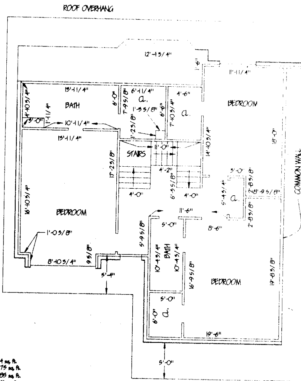
SECOND FLOOR
