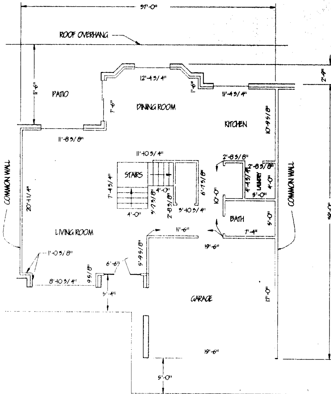
FIRST FLOOR
