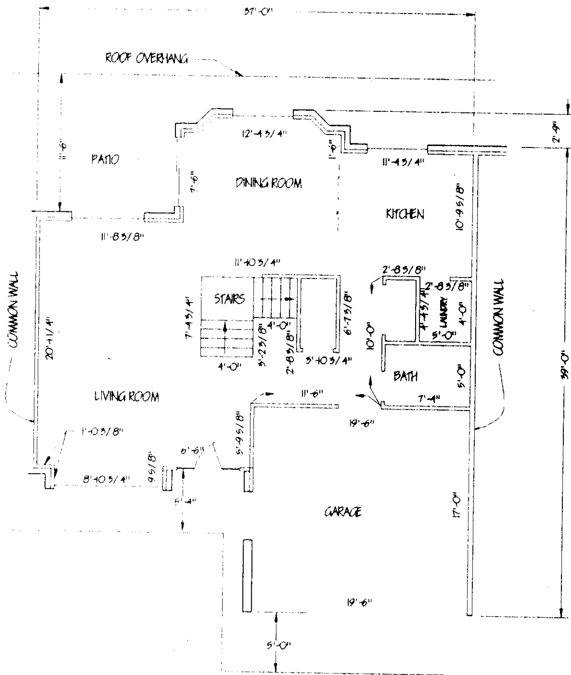
FIRST FLOOR
