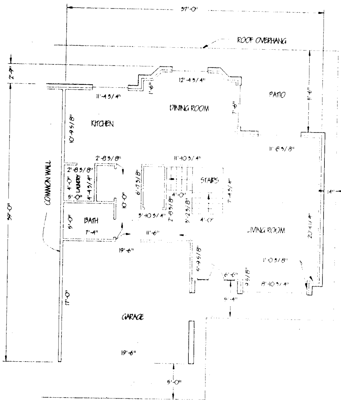
FIRST FLOOR
