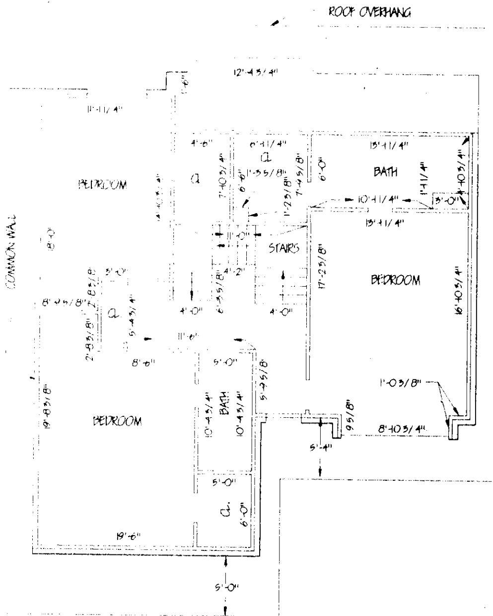
SECOND FLOOR
