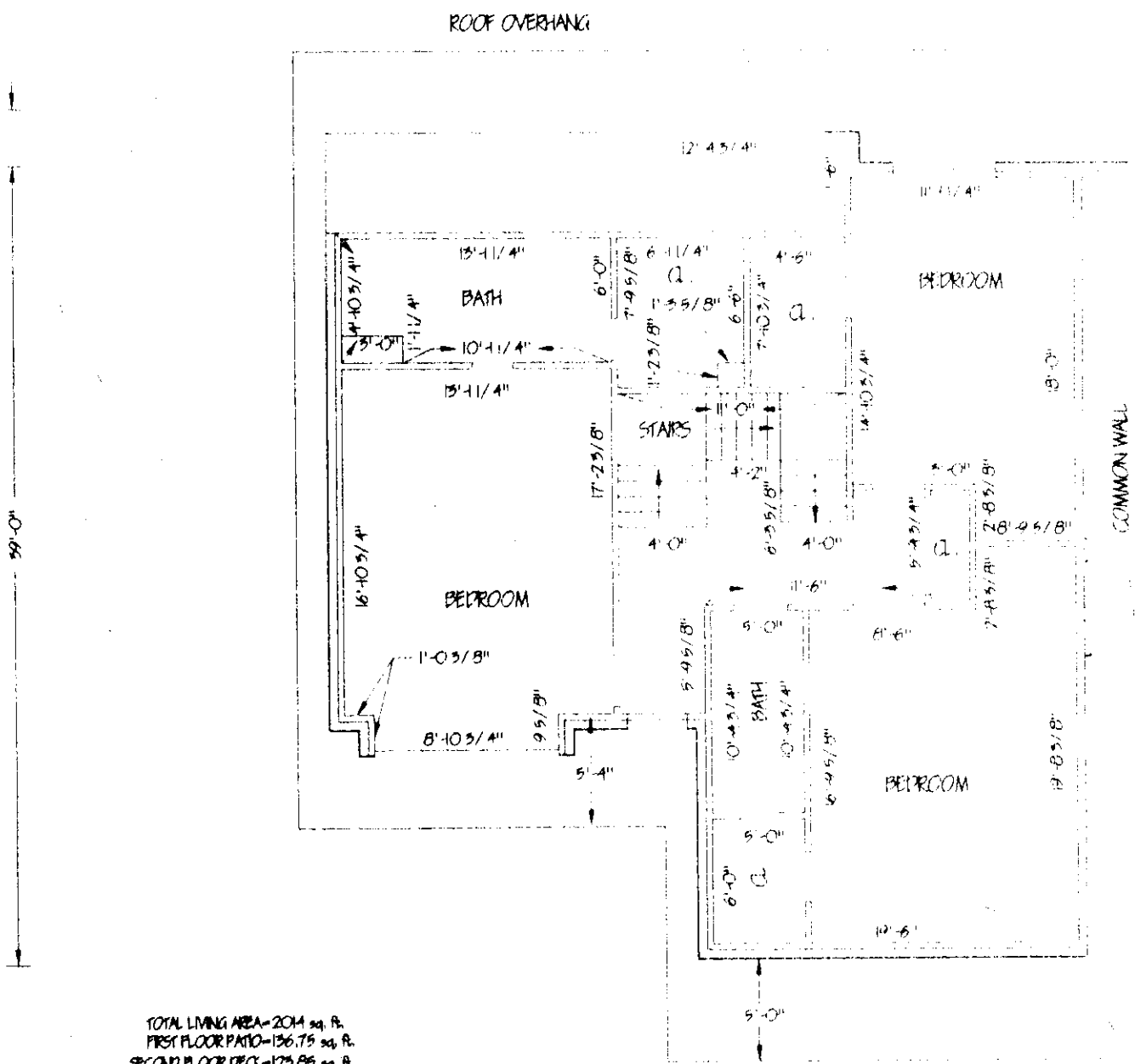
SECOND FLOOR
