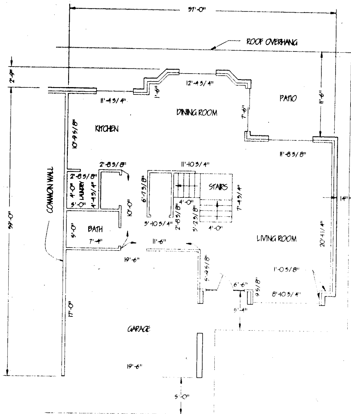
FIRST FLOOR
