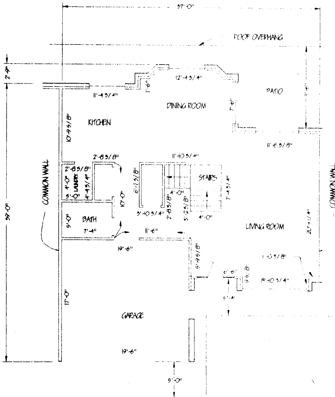
FIRST FLOOR
