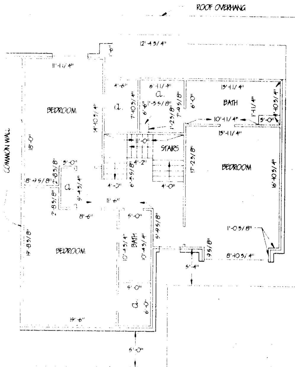
SECOND FLOOR
