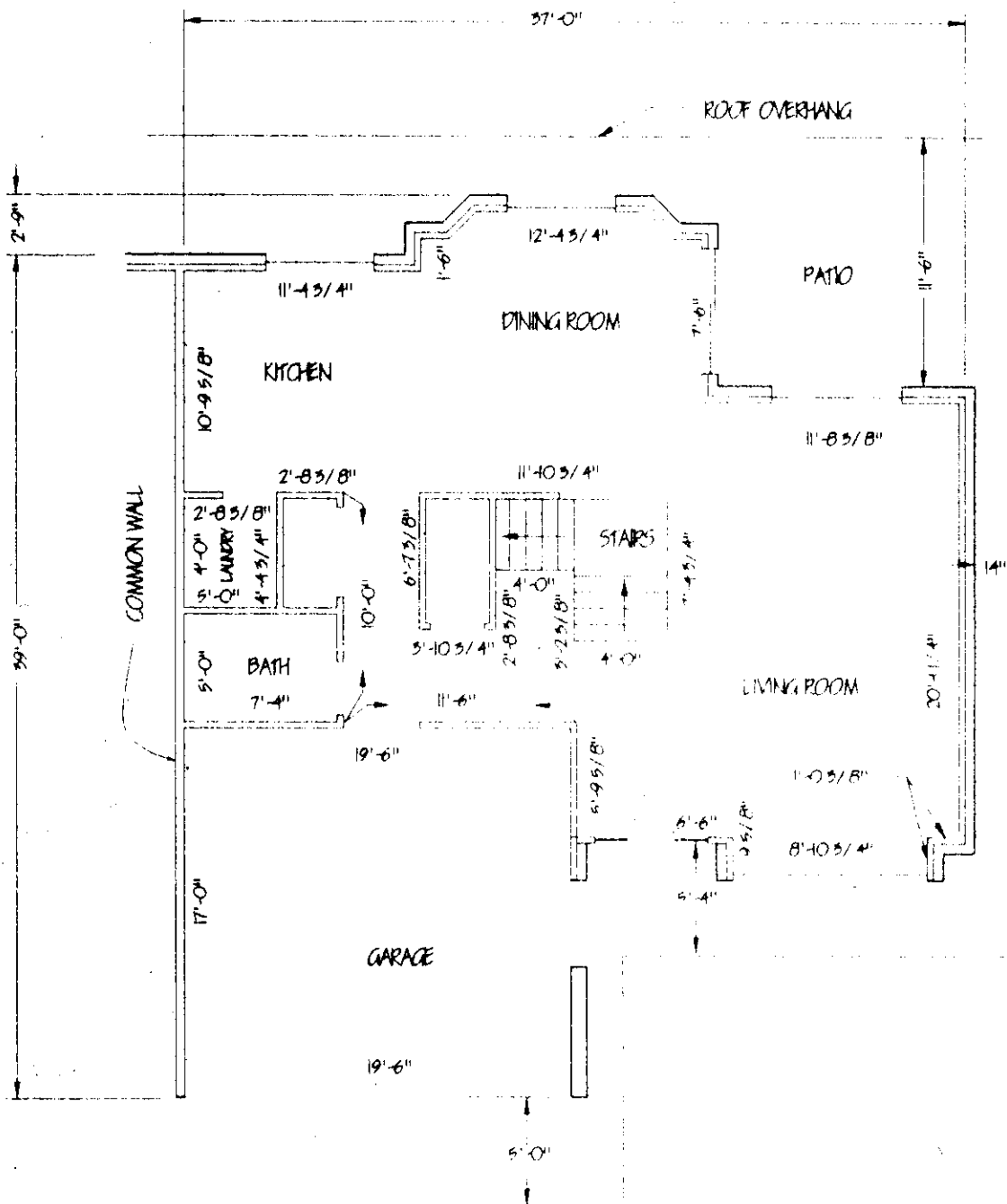
FIRST FLOOR
