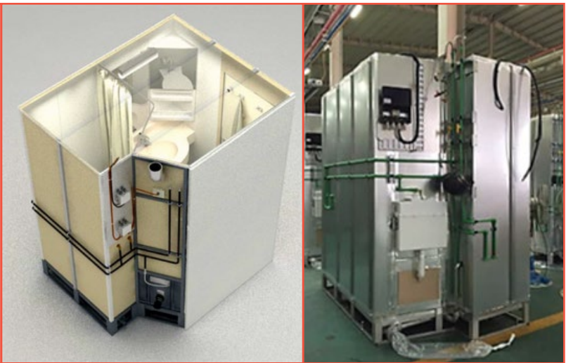
Modular toilet (Cruise Ship Cabin Quality and Grade)
