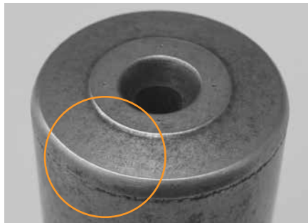
The roller end wear on this spherical bearing also was caused by fine particle contamination.
