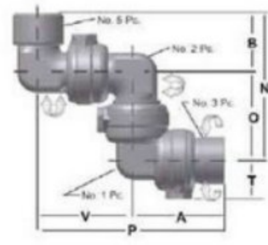
Style 80-3 Plane
