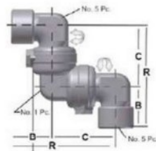
Style 70-2 Plane
