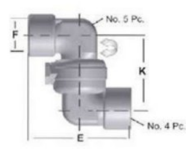
Style 40-1 Plane
