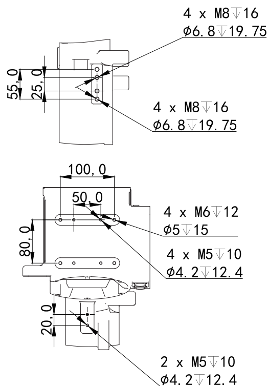
J4 motor seat installation dimensions ◀
