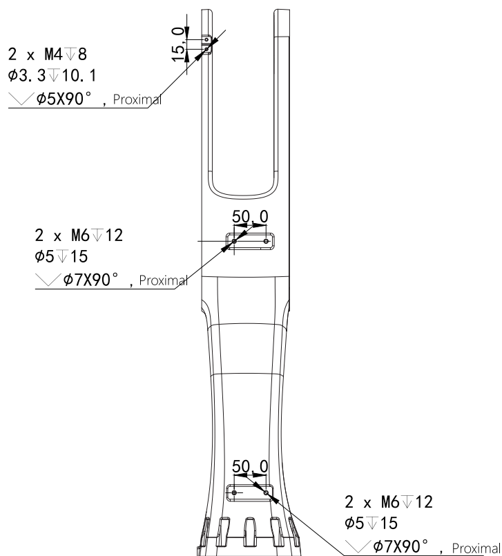
J5 wrist installation dimensions ◀
