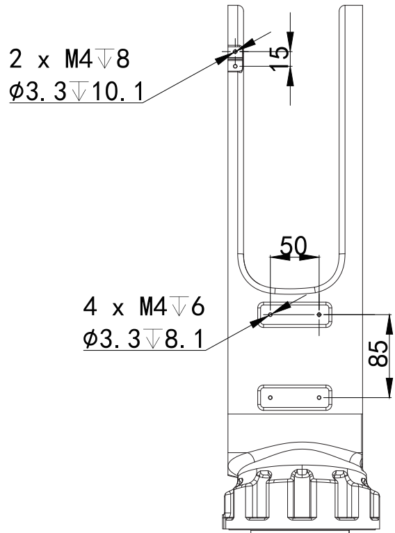
J5 wrist installation dimensions ◀
