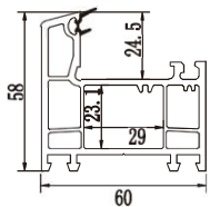
60 casement frame A
