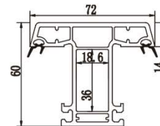
60 mullion A
