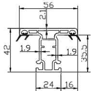
60/62/88 sliding sash mullion
