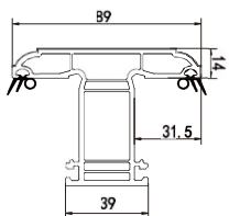
65 mullion
