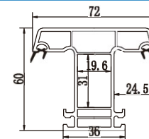
60 mullionB
