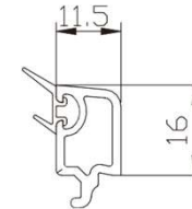
60/88 double glazing bead 11.5
