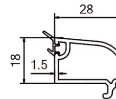
60/88 glazing bead 28
