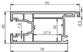
60/62/88 sliding door sash
