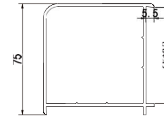
65 right angle bay corner adaptor
