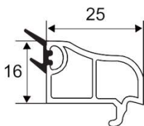
60/88 double glazing bead 25B
