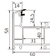
60 casement frame B
