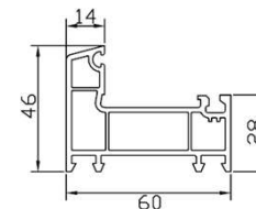
60 frame
