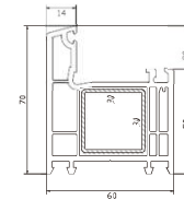
60 casement big frame
