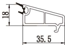
60/88 single glazing bead 35.5
