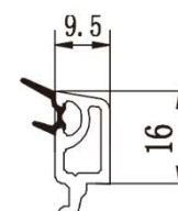
55/60/62/80/88 glazing bead 9.5
