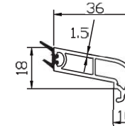
60/88 single glazing bead 36B
