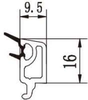
55/60/62/80/88 glazing bead 9.5
