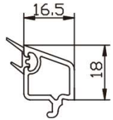
60/88 double glazing bead 16.5
