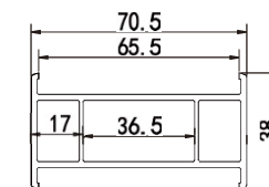
65 tube adaptor
