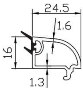
55/80 glazing bead 24.5
