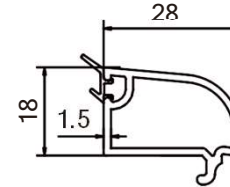
60/88 glazing bead 28
