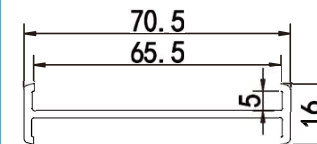
65 flat board
