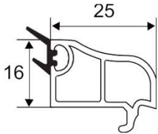
60/88 double glazing bead 25B
