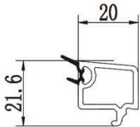
55/60/62/88/80 double glazing bead 20
