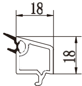
60/88 double glazing bead 18 B
