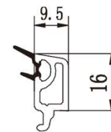
55/60/62/80/88 glazing bead 9.5
