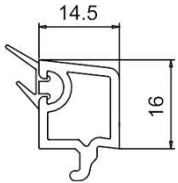
60/88 double glazing bead 14.5
