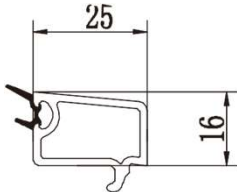
60/88 double glazing bead 25
