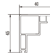
60 frame
