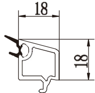
60/88 double glazing bead 18 B
