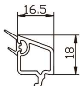
60/88 double glazing bead 16.5
