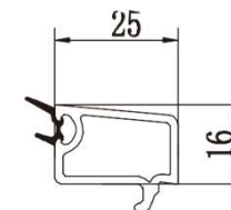
60/88 double glazing bead 25
