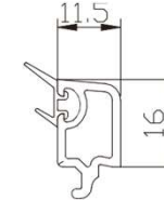
60/88 double glazing bead 11.5
