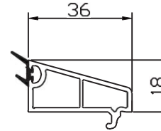
60/88 single glazing bead 36A
