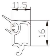
60/88 double glazing bead 11.5
