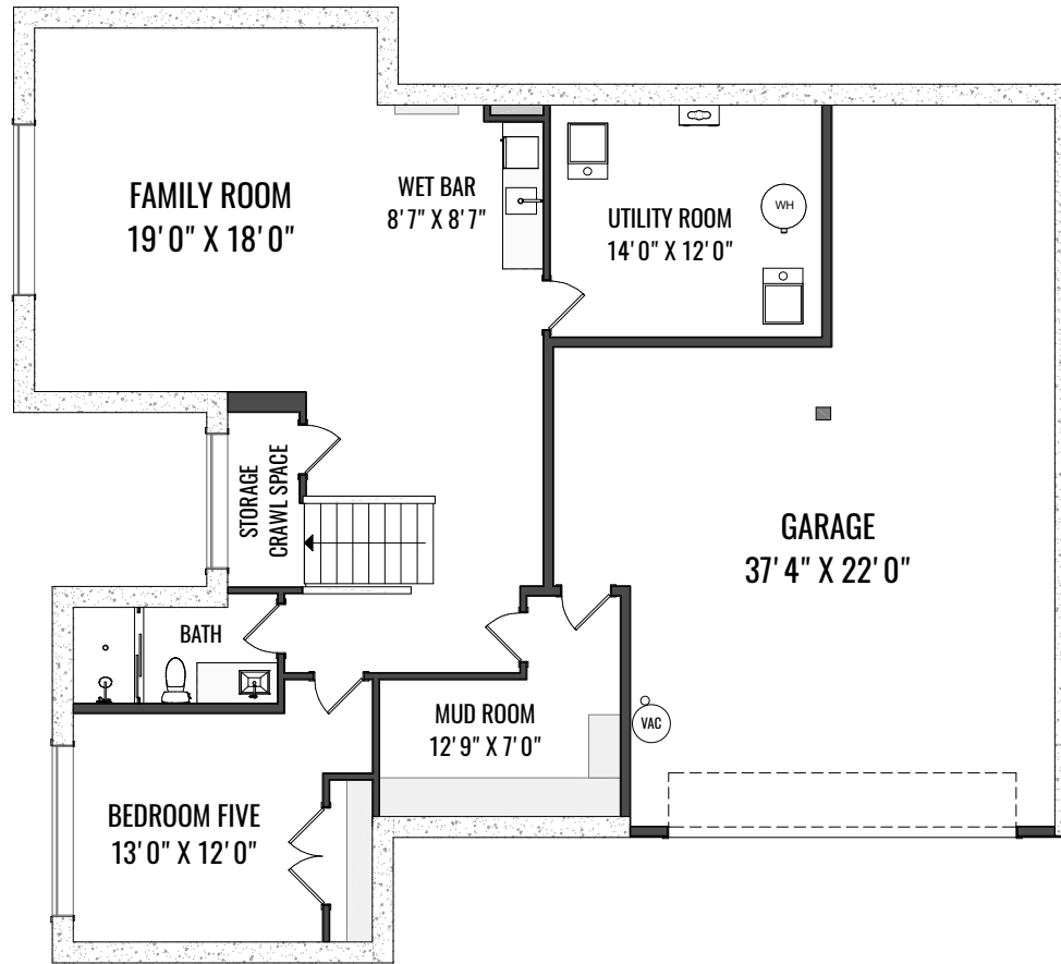
BASEMENT
