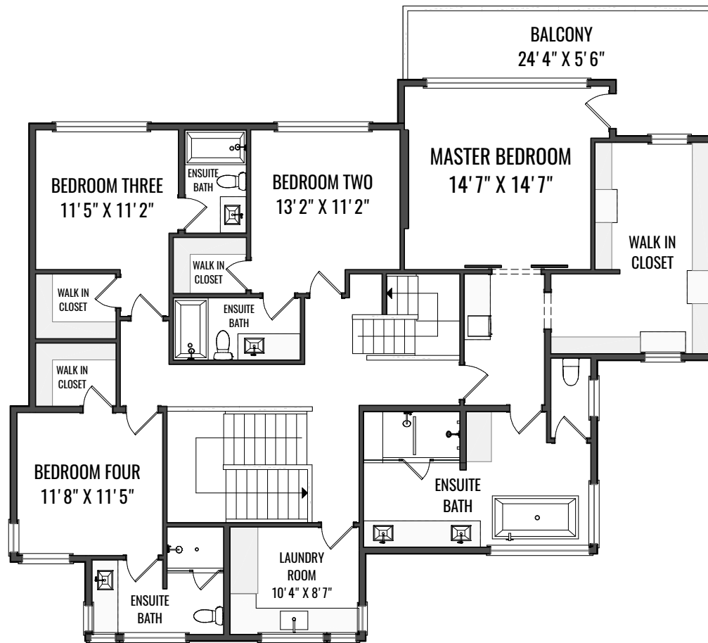
SECOND LEVEL
