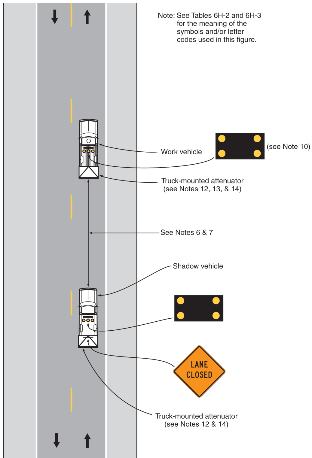
Typical Application 17
