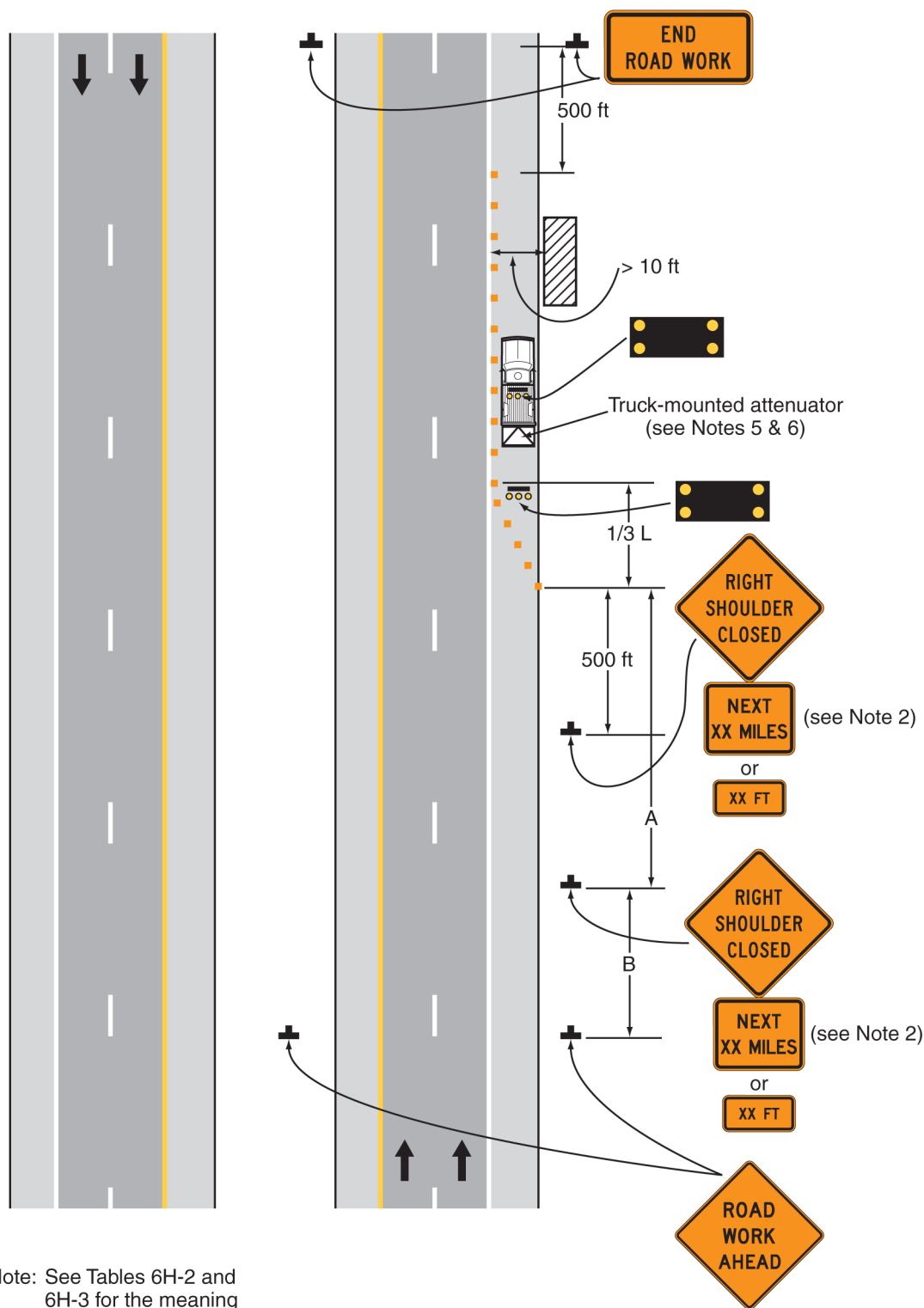
Typical Application 5A
