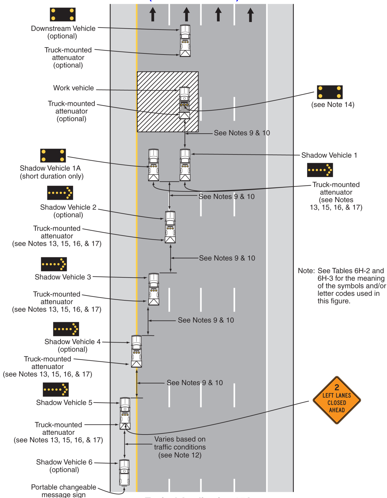
Typical Application 35A
