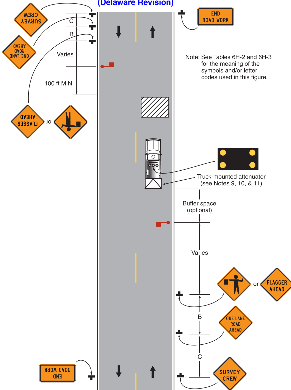
Typical Application 16
