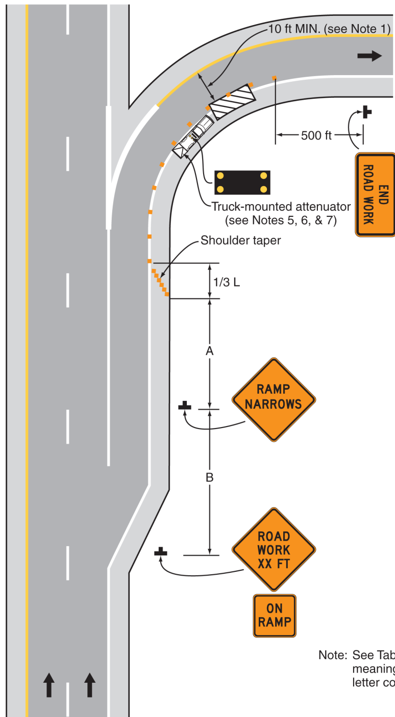
Typical Application 43
