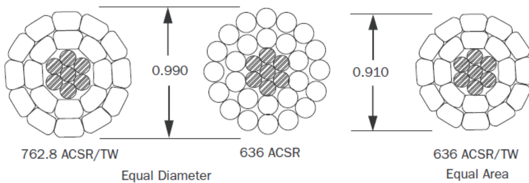
Figure 1. Comparison of ACSR and ACSR/TW conductors.
