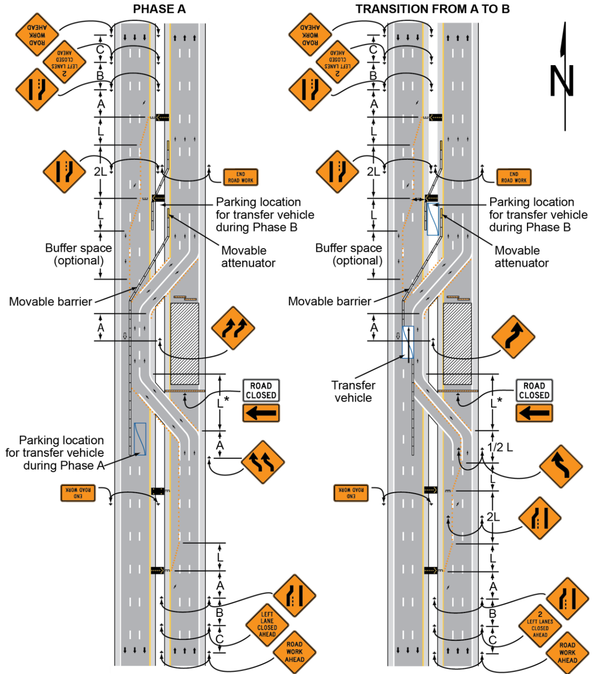
Figure 6H-45. Temporary Reversible Lane Using Movable Barriers (TA-45)
