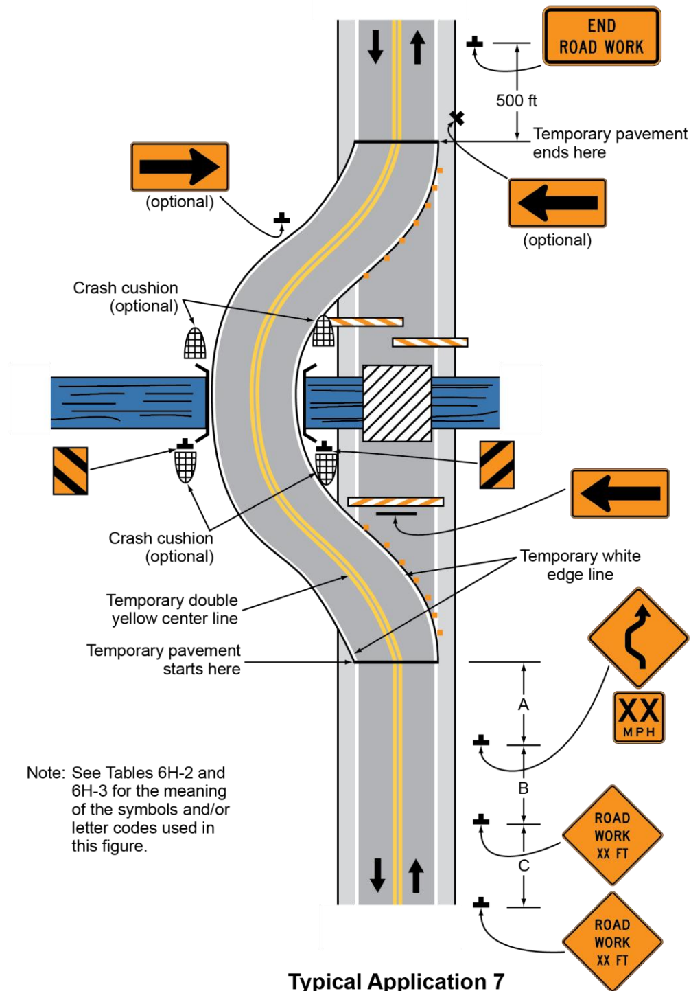
Figure 6H-7. Road Closure with a Diversion (TA-7)
