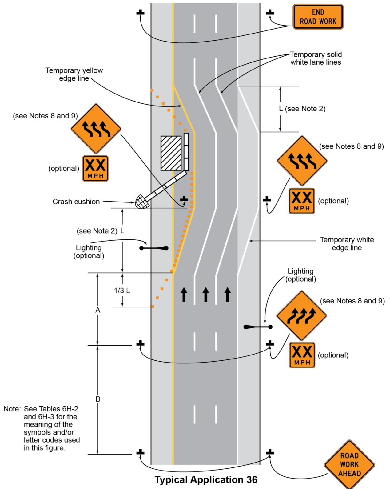
Figure 6H-36. Lane Shift on a Freeway (TA-36)
