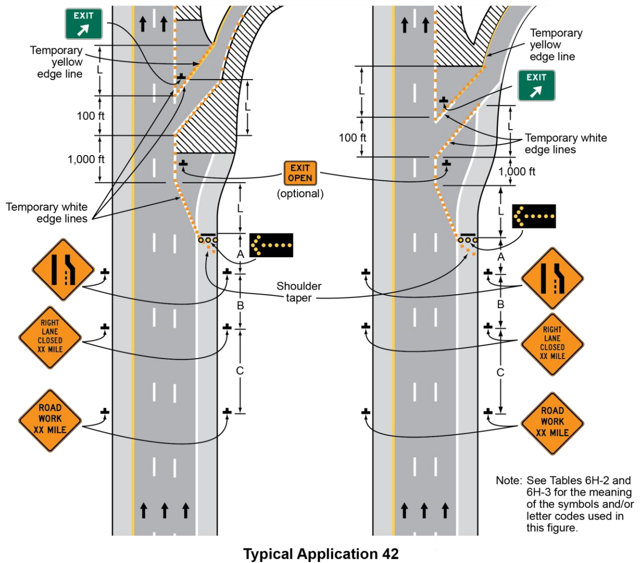
Figure 6H-42. Work in the Vicinity of an Exit Ramp (TA-42)
