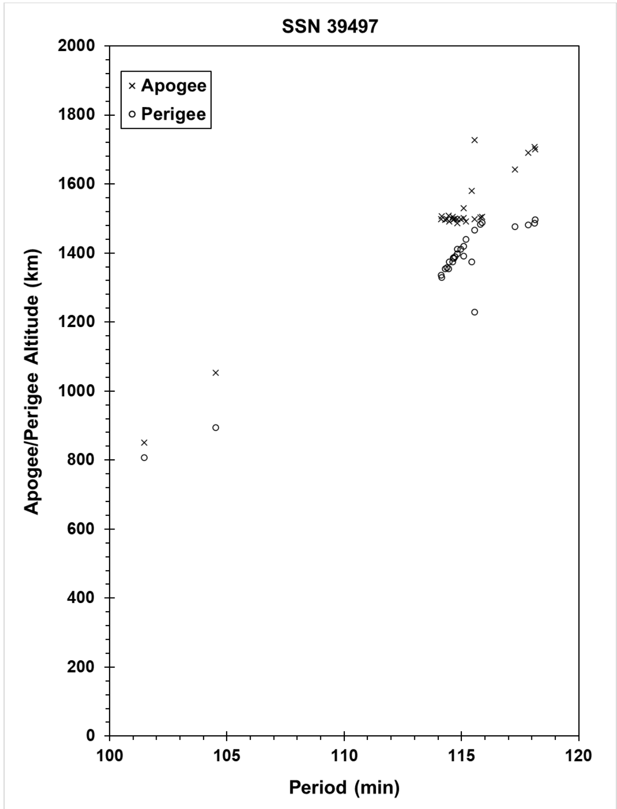
COSMOS 2491 debris cloud composed of parent spacecraft and 26 additional objects cataloged between two weeks and a year after the event. One object is likely erroneously assigned to this cloud.
