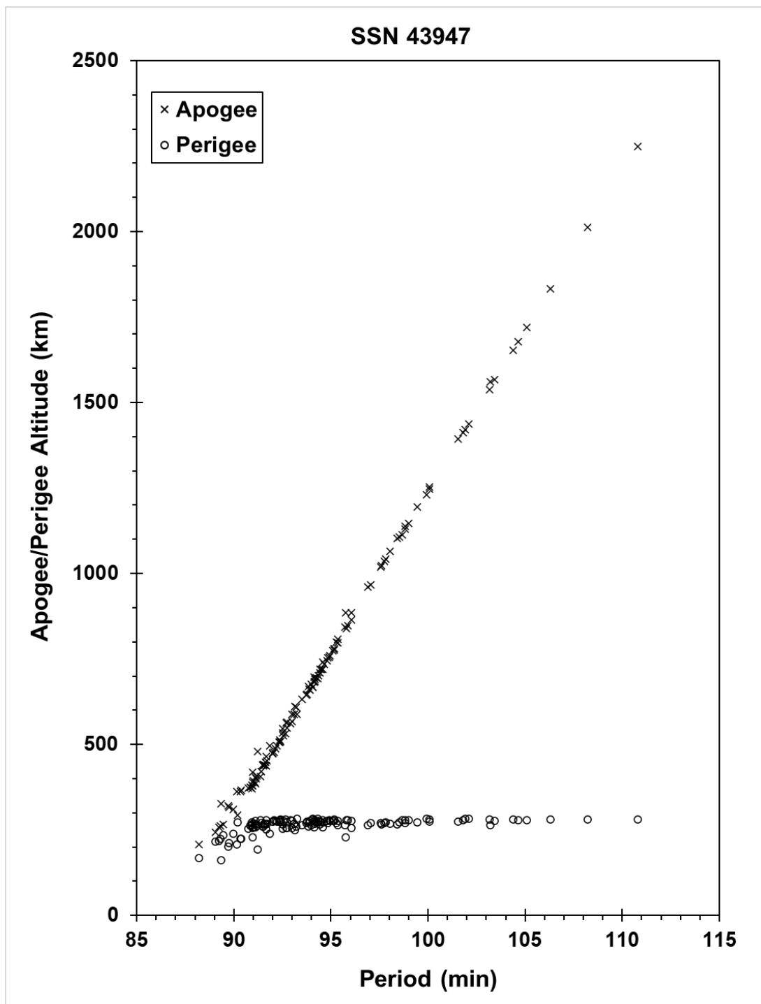
MICROSAT-R ASAT test debris cloud, composed of parent spacecraft and 128 additional objects cataloged between a week and over a year after the event.
