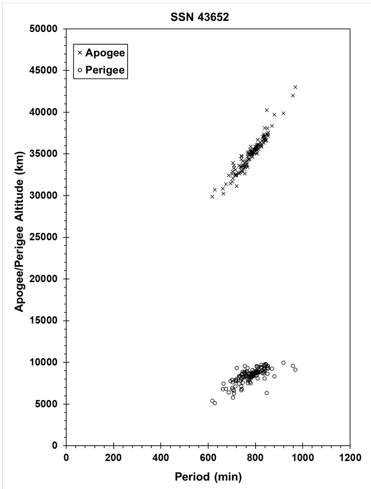
Identified Centaur V R/B debris cloud; 134 debris objects cataloged up to two years after the event as reconstructed from the US SSN database.
