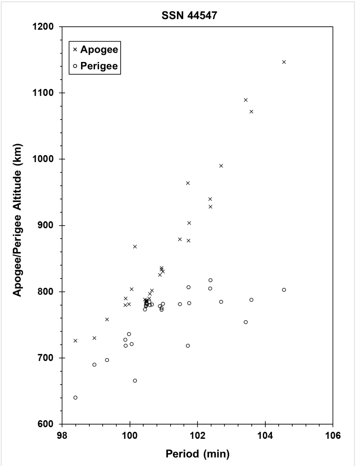
YunHai 1-02 debris cloud, composed of parent spacecraft and 29 additional objects cataloged up to approximately two months after the event.
