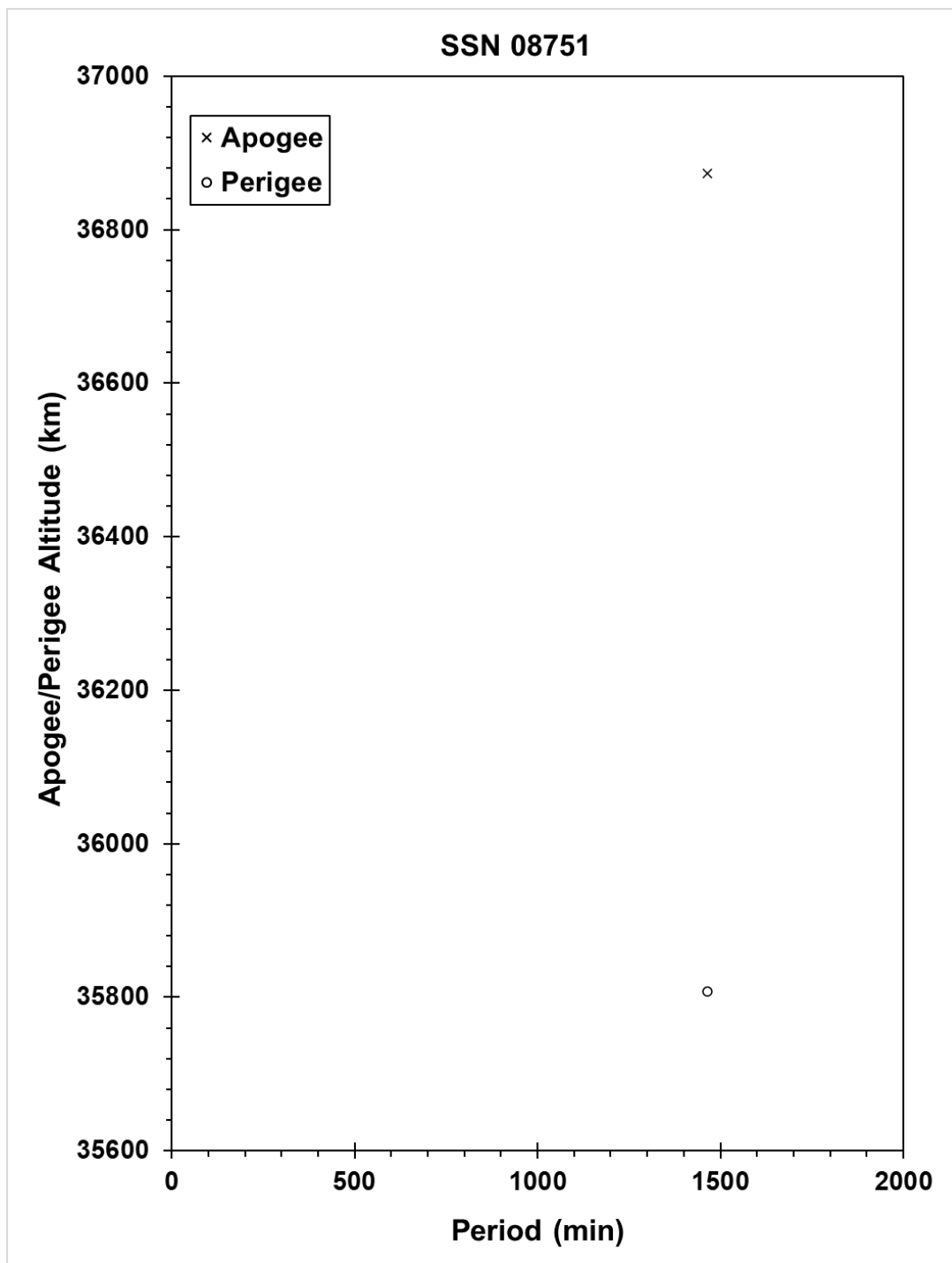
Transtase R/B debris “cloud” of parent body as reconstructed from the US SSN database.
