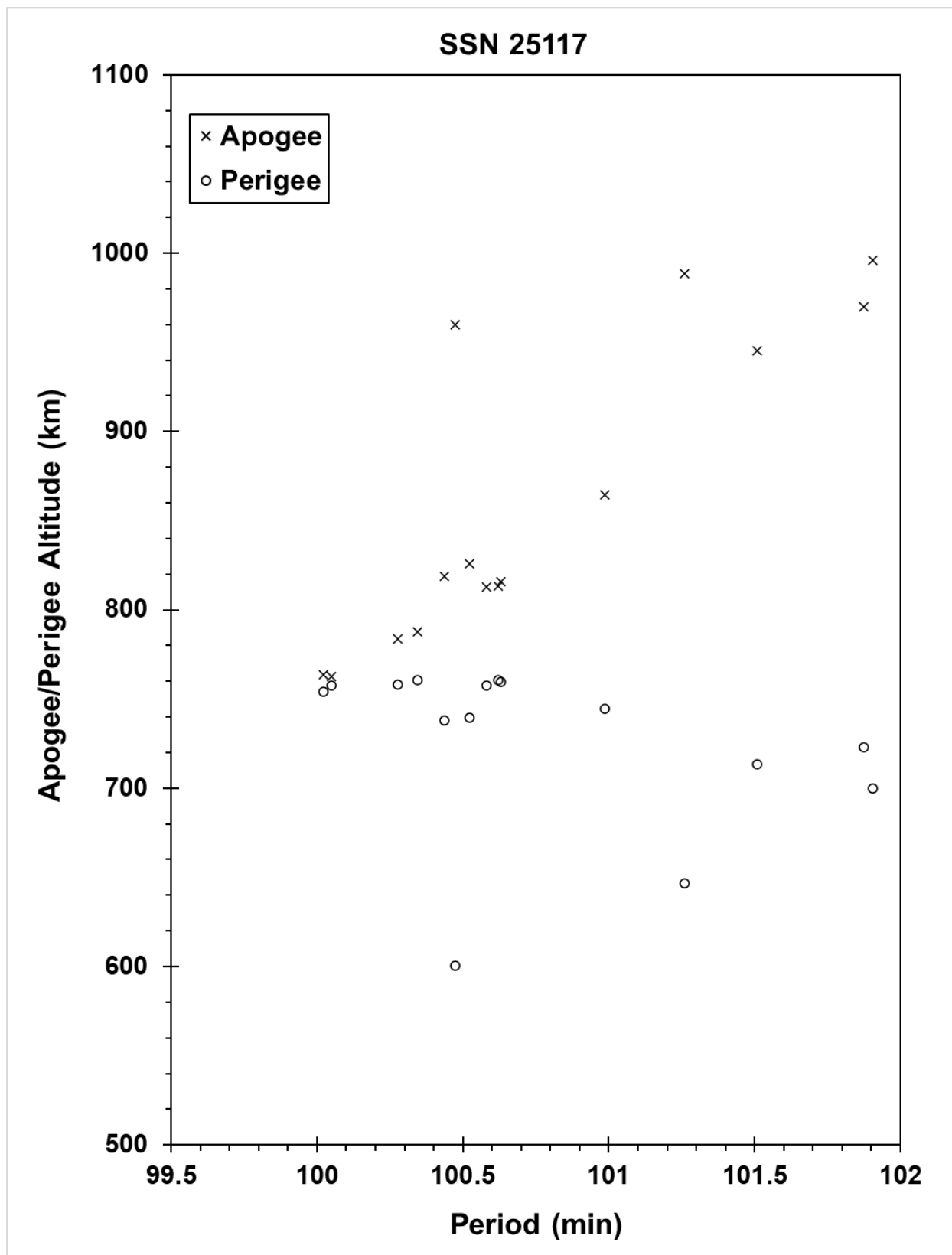
The ORBCOMM FM5 debris cloud, including 15 fragments cataloged over two months after the event.
