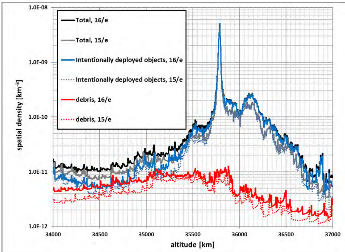
Figure 1.3.1-2. The GEO altitude population.
