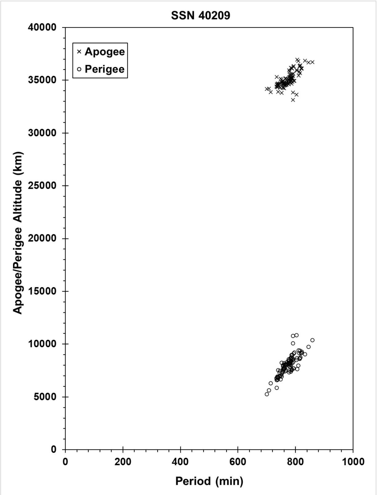
Identified Centaur V R/B debris cloud; 103 debris objects cataloged up to two years after the event as reconstructed from the US SSN database.
