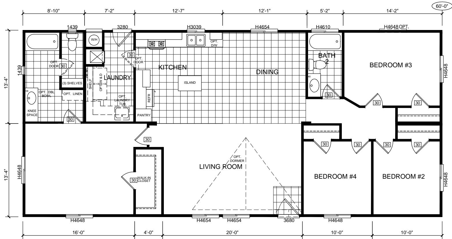
BD-09-6027 (1600 SQ. FT.) 60'-0" x 26'-8" (BEDROOM #4 OPT)
