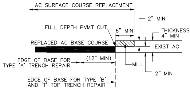
OFFSET JOINT
