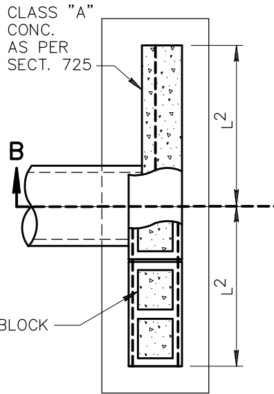
STRAIGHT TYPE
