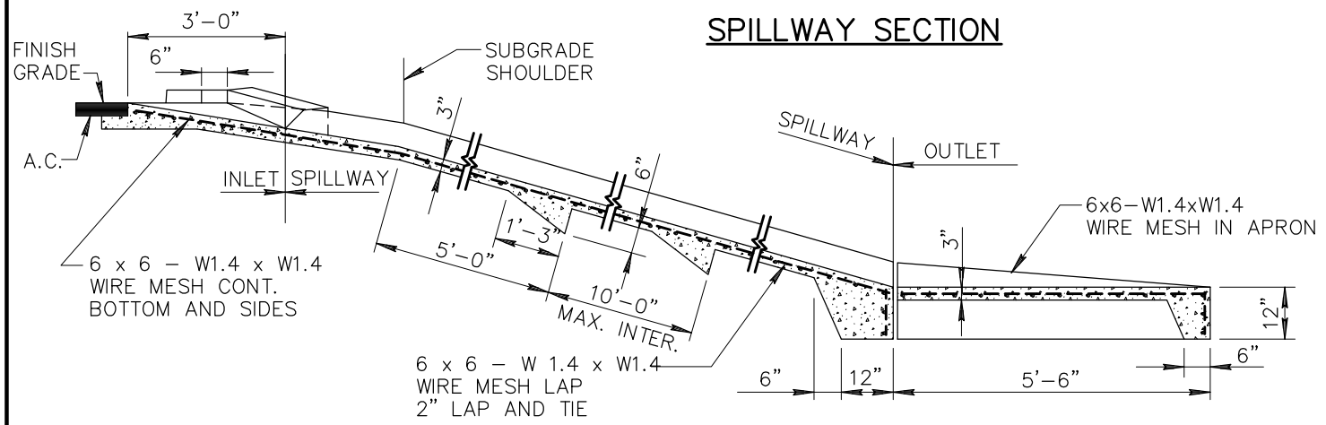
SECTION ON SPILLWAY Q DOUBLE INLET
