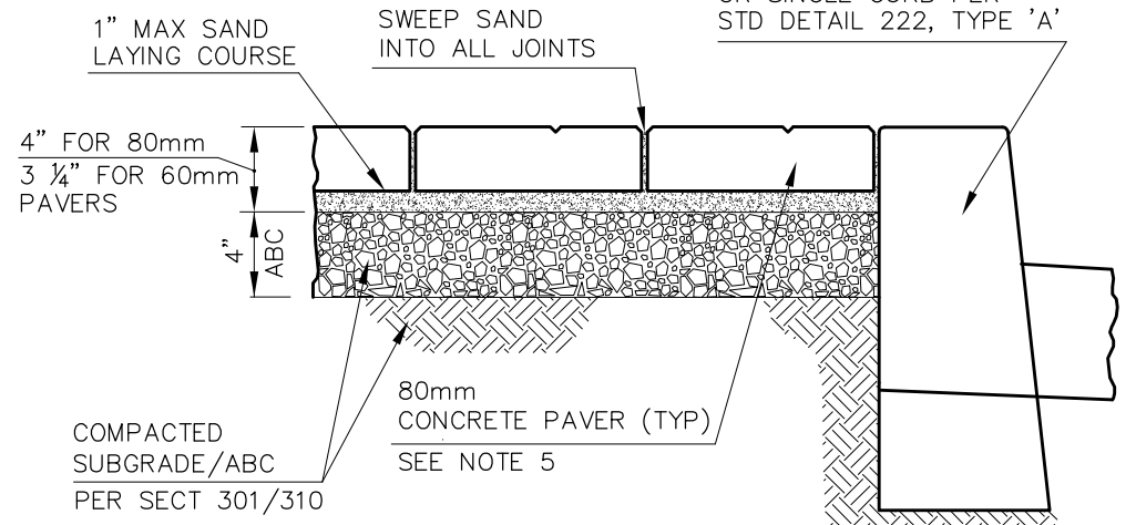
TYPICAL SECTION (RAISED MEDIAN)
