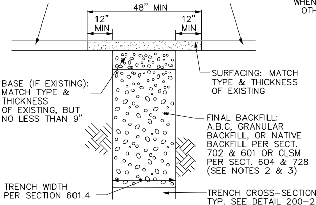
TYPE "D" TRENCH REPAIR
