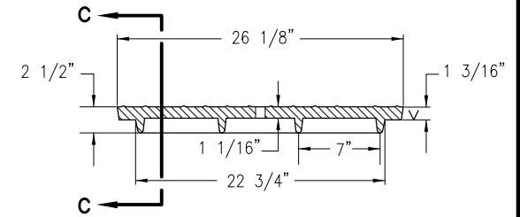
SECTION B
