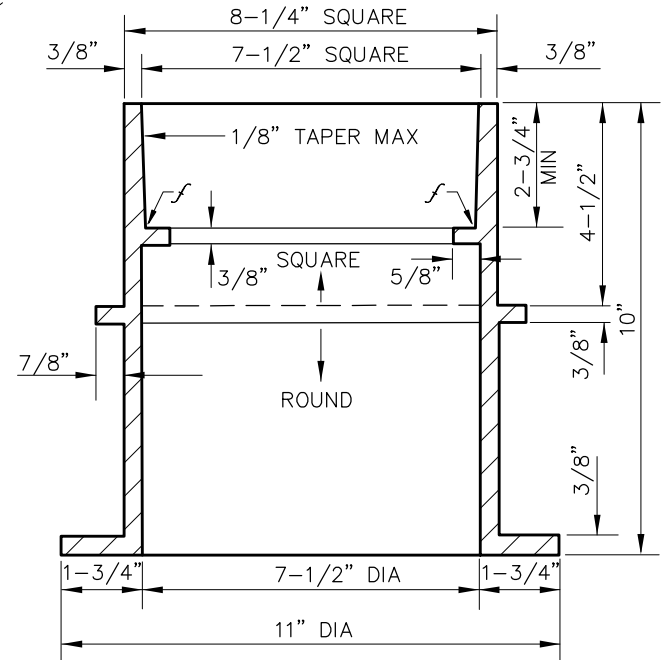
C.I. FRAME AND COVER
