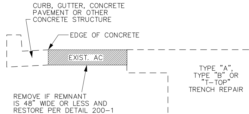
REMNANT PAVEMENT REMOVAL
