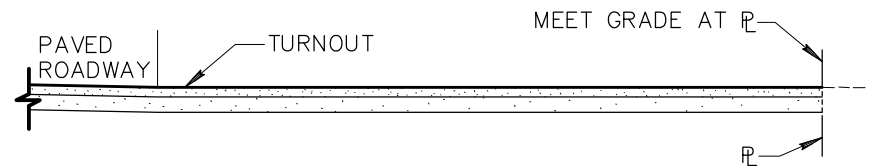
TYPICAL STRAIGHT TURNOUT
