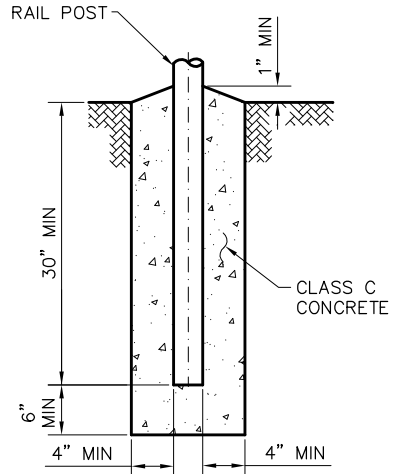
GROUND INSTALLATION DETAIL
