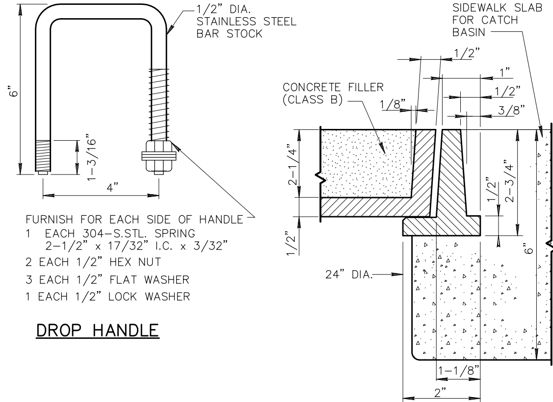
SECTION B-B
