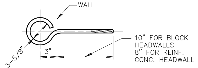
EYE BOLT
