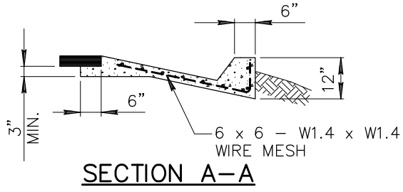
SINGLE INLET
