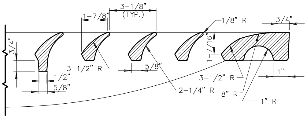
VANE DETAIL
