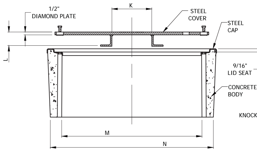
SECTION A-A BODY AND COVER
