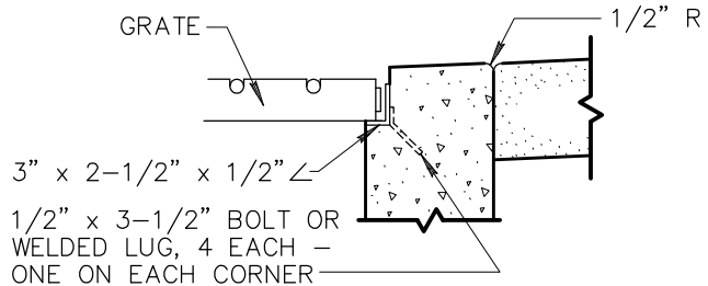
DETAIL OF ANGLE FRAME GRATE SUPPORT
