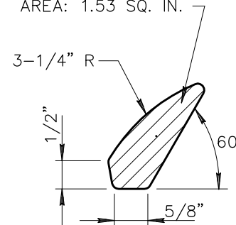
VANE DETAIL
