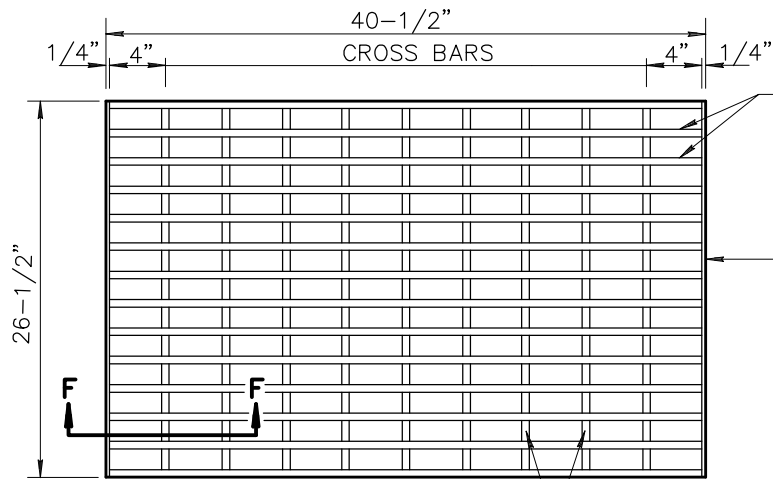
FRAME DETAIL
