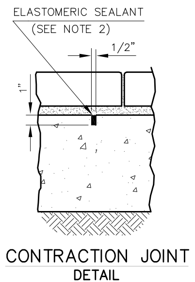
CONTRACTION JOINT DETAIL
