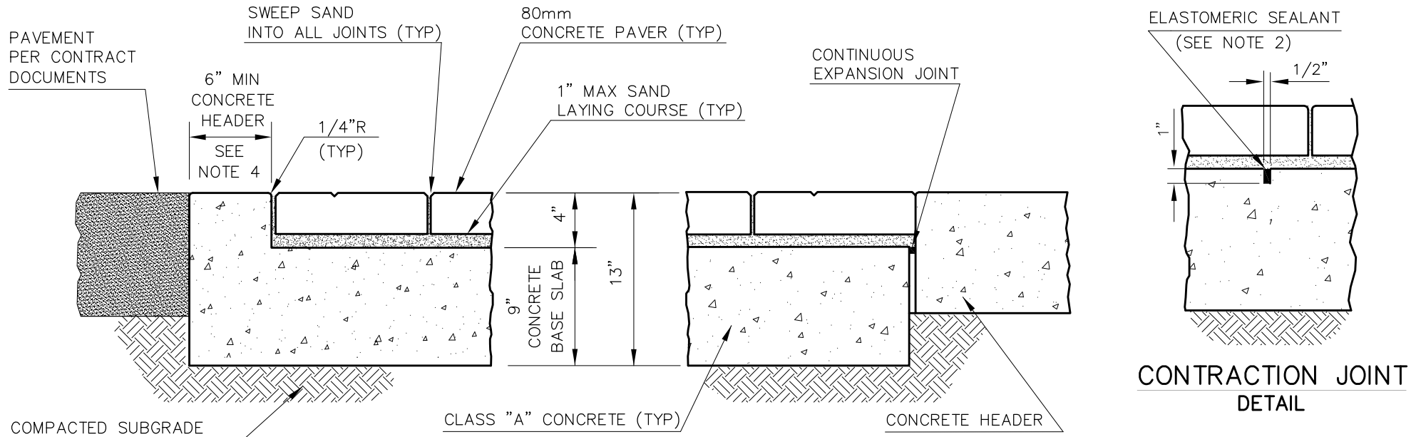
TYPICAL SECTION (AGAINST PAVEMENT)
