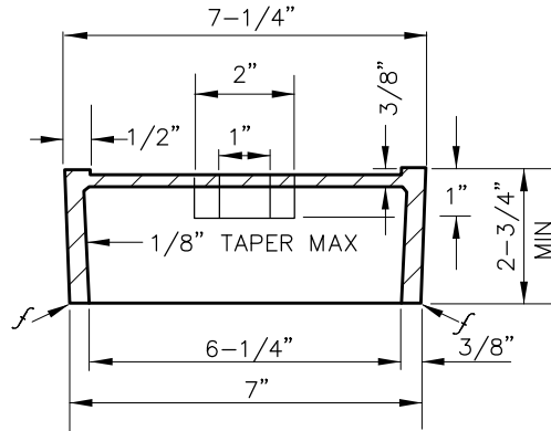
COVER SECTION A-A
