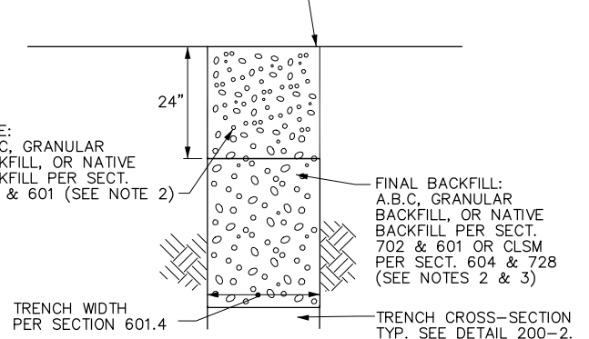
TYPE "E" TRENCH REPAIR
