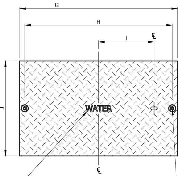
COVER ONLY - TOP VIEW
