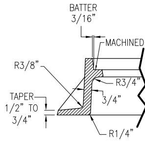
SECTION D
