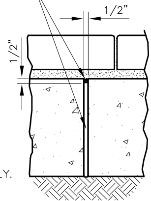
EXPANSION JOINT DETAIL
