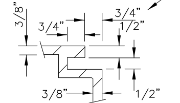
PICK HOLE SECTION
