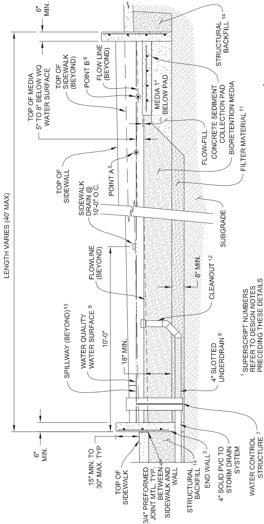
STREETSIDE BUMPOUT STORMWATER PLANTER - SECTION 2
