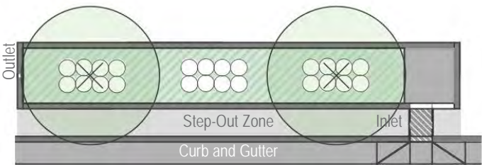
FIGURE 11. Basic Grass Cover Planting Plan (Source: Stream Design. 2015.) Scale: 1" = 10'
