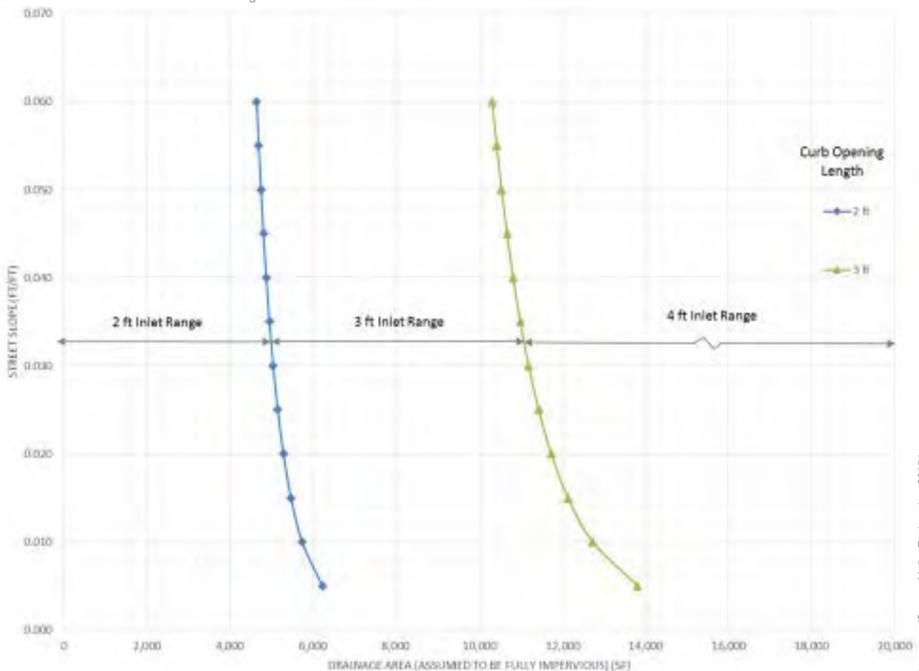
FIGURE 1. Inlet width based on drainage area.
