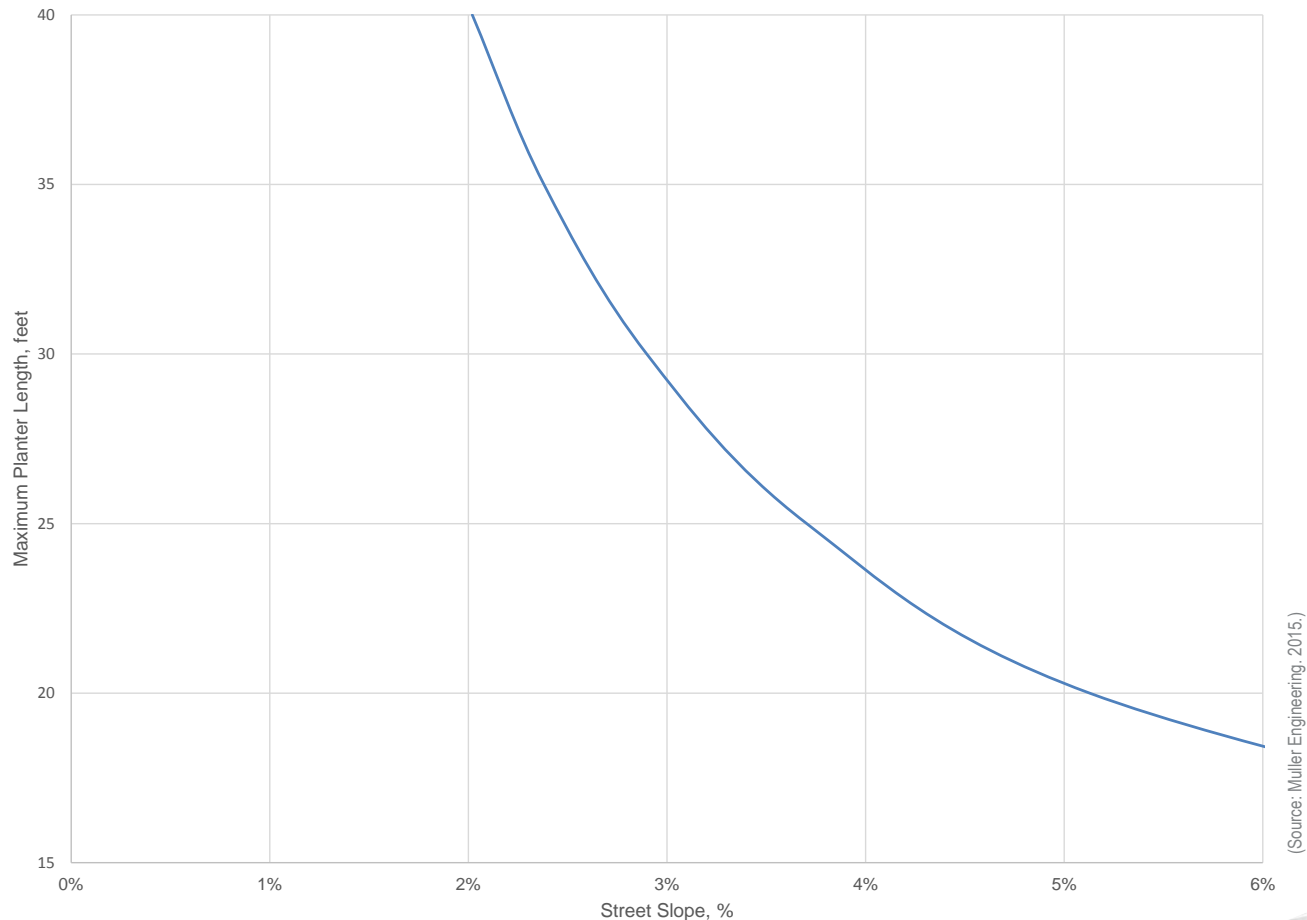
FIGURE 4. Planter length versus street slope.
