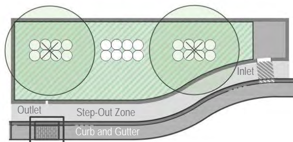
FIGURE 19. Basic Grass Cover Planting Plan (Source: Stream Design. 2015.) Scale: 1" = 10'
