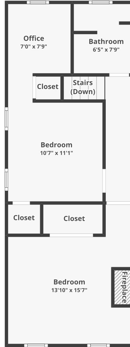
FLOOR 2
