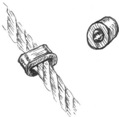
Figure 20. Loop Stop–ferrule: Aluminum ferrules can also be flattened on to the restraint cable and work well as a stop.
